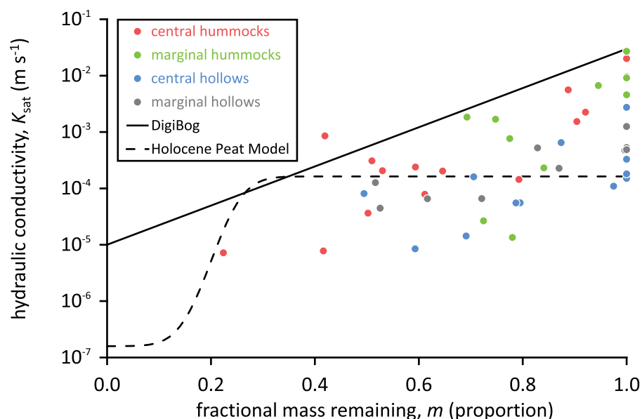
Figure 6. Relationship between C/N-derived approximation of fractional remaining mass, m , and measured saturated hydraulic conductivity. The solid and broken black lines illustrate the functions used by DigiBog (with the baseline parameterization used by Morris et al. [2011]) and the Holocene Peat Model (with the baseline parameterization given by Frolking et al. [2010]), respectively, to simulate hydraulic conductivity on the basis of fractional remaining mass.
