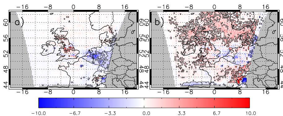
Figure 5. Mean bias in tropospheric NO 2 column ( \times 10^{15} molecules \text{cm}^{-2} ), 2006, between AQUM Run C (AKs applied) and OMI for (a) summer (RMSE = 3.68 \times 10^{15} molecules \text{cm}^{-2} and FGE = 0.65) and (b) winter (RMSE = 5.12 \times 10^{15} molecules \text{cm}^{-2} and FGE = 0.63). The RMSE and FGE are over the UK between 8^\circ W– 2^\circ E and 50 – 60^\circ N and black polygoned regions show significant differences. Also the same for mean bias plots in Figs. 6–9.
