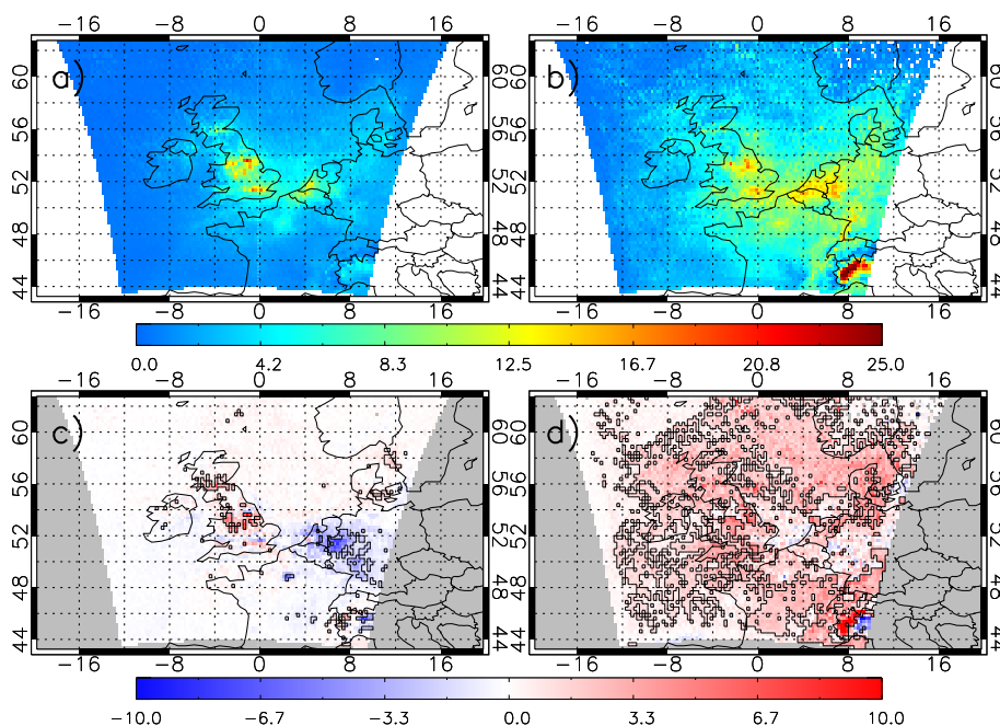
Figure 6. Tropospheric NO 2 column ( \times 10^{15} molecules \text{cm}^{-2} ), 2006, from AQUM Run MACC (AKs applied) for (a) summer and (b) winter. AQUM Run MACC (AKs applied) and OMI mean bias for (c) summer (RMSE = 3.74 \times 10^{15} molecules \text{cm}^{-2} and FGE = 0.63) and (d) winter (RMSE = 6.00 \times 10^{15} molecules \text{cm}^{-2} and FGE = 0.65).
