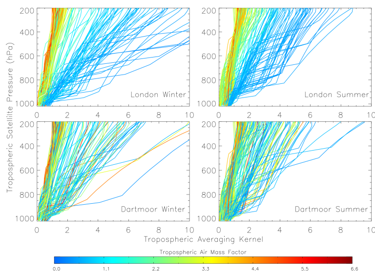
Figure 1. Example OMI averaging kernels for London (top) and Dartmoor (bottom) for summer (right) and winter (left) 2006. Averaging kernels have been coloured according to their respective tropospheric air mass factor values.
