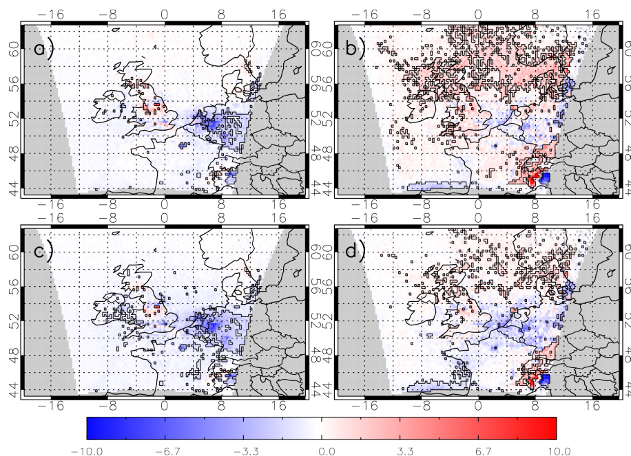
Figure 9. MB in tropospheric NO 2 column ( \times 10^{15} molecules \text{cm}^{-2} ), 2006, between AQUM (AKs applied)–OMI for (a) summer \gamma = 0.001 (RMSE = 3.39 \times 10^{15} molecules \text{cm}^{-2} and FGE = 0.65), (b) winter \gamma = 0.001 (RMSE = 5.05 \times 10^{15} molecules \text{cm}^{-2} and FGE = 0.62), (c) summer \gamma = 0.02 (RMSE = 3.08 \times 10^{15} molecules \text{cm}^{-2} and FGE = 0.67) and (d) winter \gamma = 0.02 (RMSE = 4.48 \times 10^{15} molecules \text{cm}^{-2} and FGE = 0.60).
