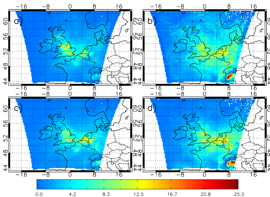
Figure 4. Tropospheric NO 2 column ( \times 10^{15} molecules \text{cm}^{-2} ), 2006, for (a) AQUM Run C (with averaging kernels (AK) applied) summer, (b) AQUM Run C (AKs applied) winter, (c) OMI summer and (d) OMI winter.
