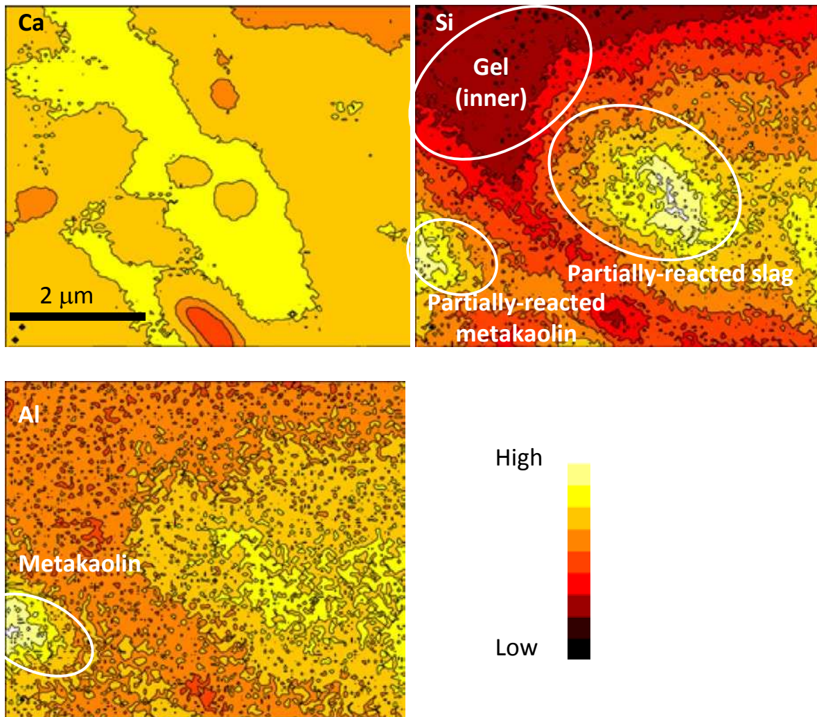
Figure 4. X-ray fluorescence micrographs of a sodium silicate-activated binder (80% slag/20% metakaolin, activator \text{SiO}_2/\text{Na}_2\text{O} ratio 0.9). The maps were obtained with a focused 10.5 keV X-ray beam with a spot size of 50 nm, and a step size of 50 nm. The same region is shown in all parts of the Figure. Data were collected using beamline 26-ID (Hard X-ray Nanoprobe), operated by the Center for Nanoscale Materials at the Advanced Photon Source, Argonne National Laboratory, Illinois, USA.
