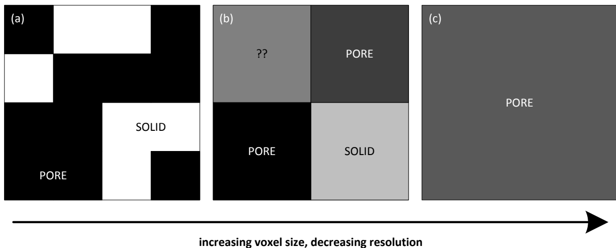
Figure 6. The distinction between pore space and binder phase becomes more difficult as voxel size is increased above the fundamental pore size, for an arbitrary pore geometry. As the voxel size increases, the likelihood of error associated with segmentation increases; in (a) it is clear what is pore and what is solid, whereas in (b) and (c) it becomes increasingly more difficult to distinguish the pore and solid phases.
