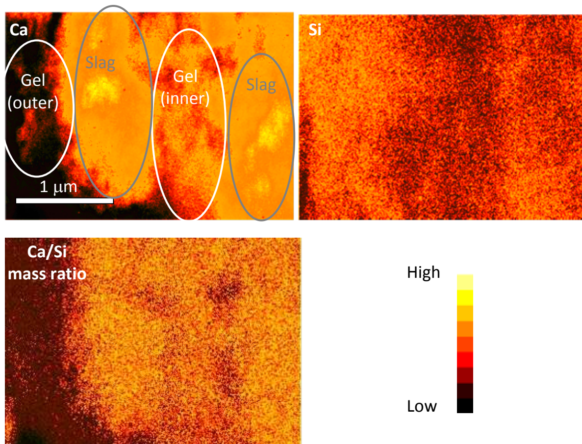
Figure 3. X-ray fluorescence micrographs of a sodium metasilicate-activated binder (75% slag/25% metakaolin, activator \text{SiO}_2/\text{Na}_2\text{O} ratio 1.0). The maps were obtained with a focused 12 keV X-ray beam with a spot size of 50 nm, and a step size of 10 nm. The same region is shown in all parts of the Figure; the gel and slag regions are identified in the Ca map only. Data were collected using beamline 26-ID (Hard X-ray Nanoprobe), operated by the Center for Nanoscale Materials at the Advanced Photon Source, Argonne National Laboratory, Illinois, USA.
