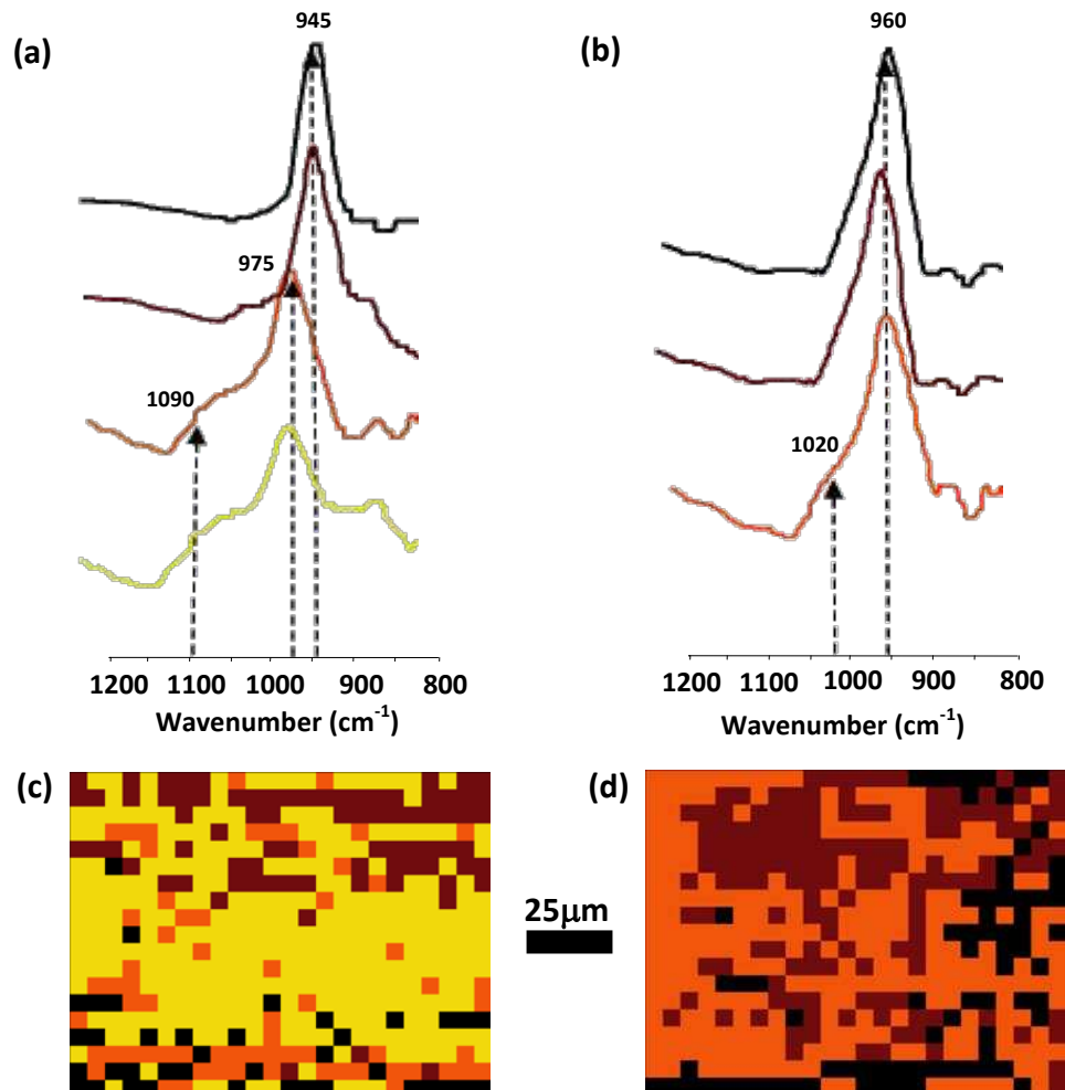
Figure 1. Synchrotron infrared microscopy data for geothermal silica-sodium aluminate geopolymer binders, without (a,c) and with (b,d) 0.5 wt.% nano- \text{Al}_2\text{O}_3 seeding. Hierarchical clustering of the spectra obtained at each point results in the cluster spectra shown in (a) and (b), and the distributions of the spectra on the samples are shown in (c) and (d). Data from [14], collected using the Infrared beamline of the Australian Synchrotron, Clayton, Victoria, Australia, in attenuated total reflectance geometry using a diamond crystal probe.
