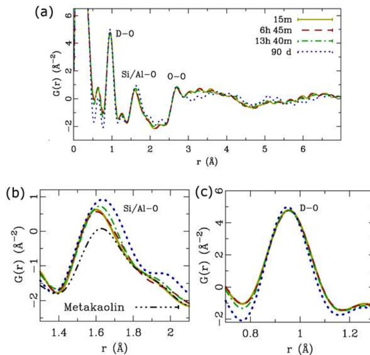
Figure 2. In situ neutron pair distribution functions of a deuterated sodium silicate-activated metakaolin geopolymer, obtained after reaction times as marked, at ambient temperature ( 25^{\circ}\text{C} ). Parts (b) and (c) are expansions of key peaks in (a), and (b) shows a comparison to the pair distribution function of the raw metakaolin used in geopolymer synthesis. Data from [21], collected using the HIPD instrument at the Lujan Neutron Scattering Center, Los Alamos National Laboratory, New Mexico, USA.
