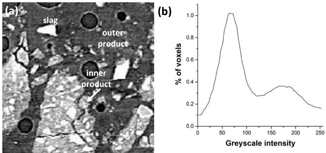
Figure 5. (a) One slice from an X-ray microtomography scan of a sodium silicate-activated binder (80% slag/20% metakaolin, activator \text{SiO}_2/\text{Na}_2\text{O} ratio 0.9), field of view 150 \times 150 \mu\text{m} , and (b) a grayscale histogram of the volume of interest. Data were collected on beamline 2-BM-B at the Advanced Photon Source, Argonne National Laboratory, Illinois, USA, using 22.5 keV radiation.
