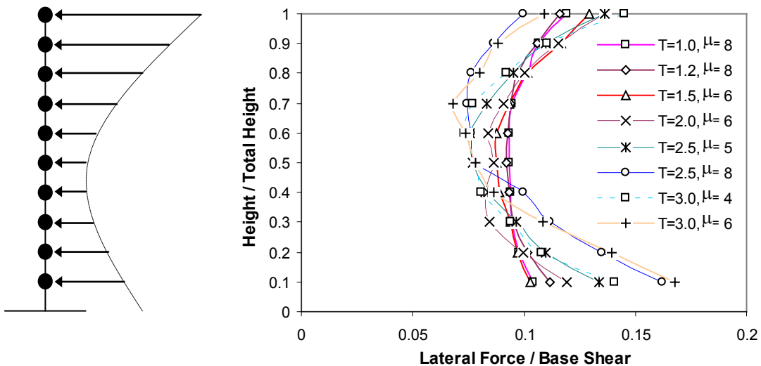
Figure 11: Hyperbolic load pattern
