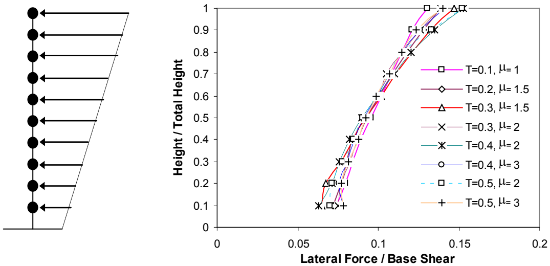
Figure 9: Trapezoid load patterns
