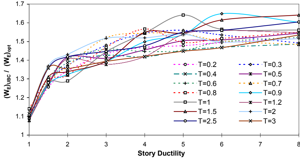
Figure 6: The ratio of total structural weight for the UBC designed models to the optimum models, (W_E)_{UBC} / (W_E)_{opt} , Average of 20 earthquakes
