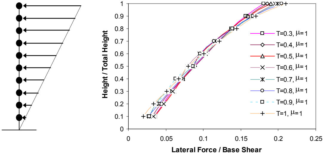
Figure 8: Triangular load patterns
