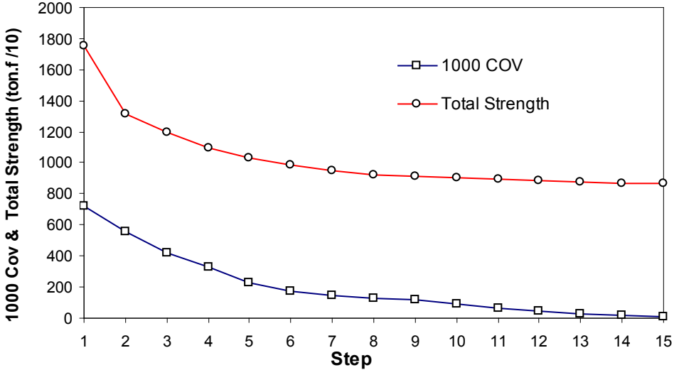
Figure 3: Cov of story ductility demands and total story strength for feasible answers, 10-story shear building with T=1 Sec and \mu_{ti}=4 , Northridge 1994 (CNP196)
