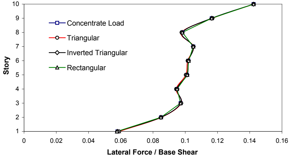
Figure 5: Optimum load pattern for different initial strength distributions, 10-story shear building with T=1 Sec and \mu_{ti}=4 , Northridge 1994 (CNP196)
