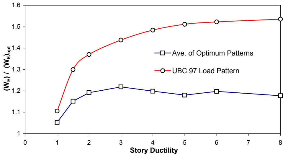
Figure 7: The ratio of required structural weight to the optimum weight, (W_E) / (W_E)_{opt} , for the models designed with the average pattern and those designed conventionally, Average of 20 earthquakes
