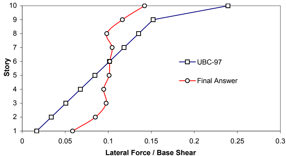
Figure 4: Comparison of UBC-97 & optimum lateral force distribution, 10-story shear building with T=1 Sec and \mu_{ti}=4 , Northridge 1994 (CNP196)
