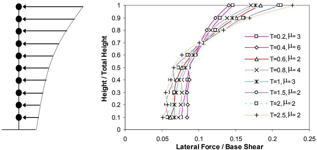
Figure 10: Parabolic load patterns
