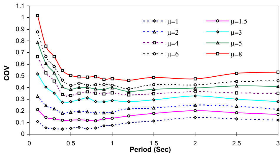
Figure 2: Cov of story ductility demands, average of 20 earthquakes
