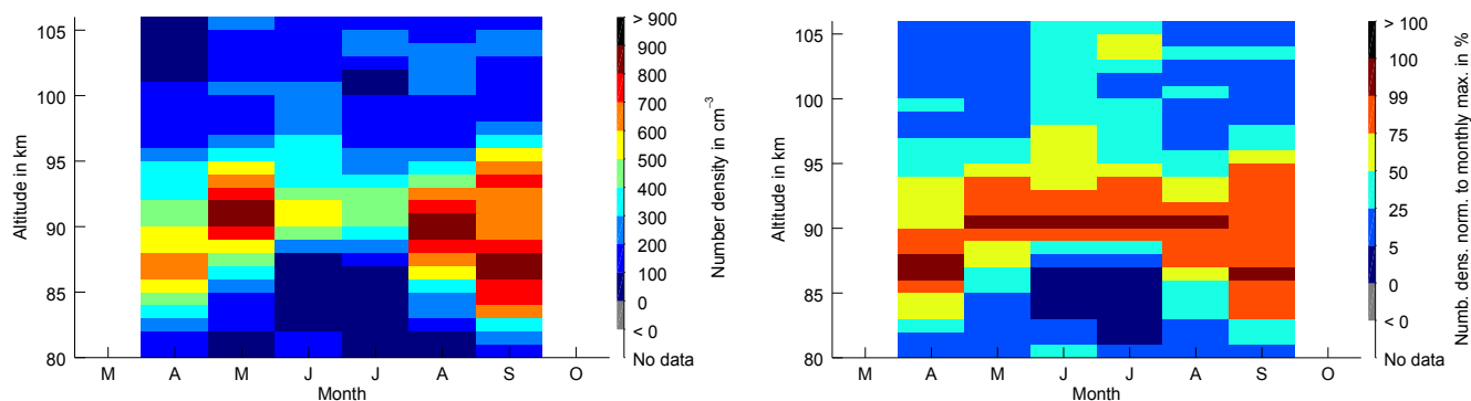
Figure 22. Vertical profile of Mg density (left) and Mg density normalized to the monthly maximum (right) at 70° N, a latitude observed with SCIAMACHY before, during and after the period when NLCs occur. NLCs occur at this latitude between about the end of May and mid-August.
