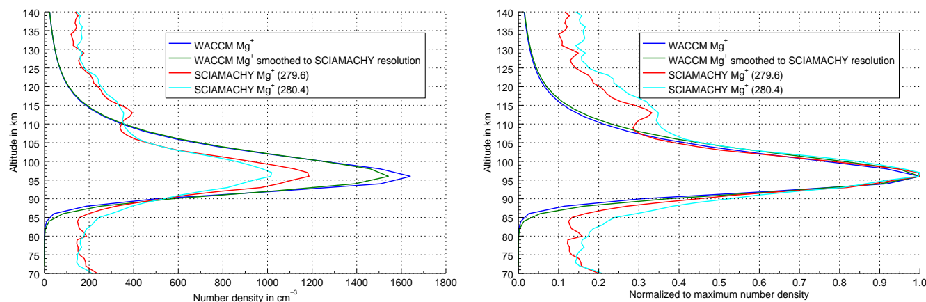
Figure 20. Vertical profiles of \text{Mg}^+ for SCIAMACHY and WACCM at the equator. The right plot shows the profiles normalized to the maximum of each profile, to better compare the shape of the profiles. The VCD between 70 and 140 km at the equator is 2.7 \times 10^9 \text{ cm}^{-2} for SCIAMACHY (both 279.6 nm and 280.4 nm) and 2.4 \times 10^9 \text{ cm}^{-2} for WACCM. Note that the statistical error for SCIAMACHY estimated by (Langowski et al., 2013) (Figs. 22 and 23) is \approx \pm 150 \text{ cm}^{-3} for the 279.6 nm line and \approx \pm 250 \text{ cm}^{-3} for the 280.4 nm line.
