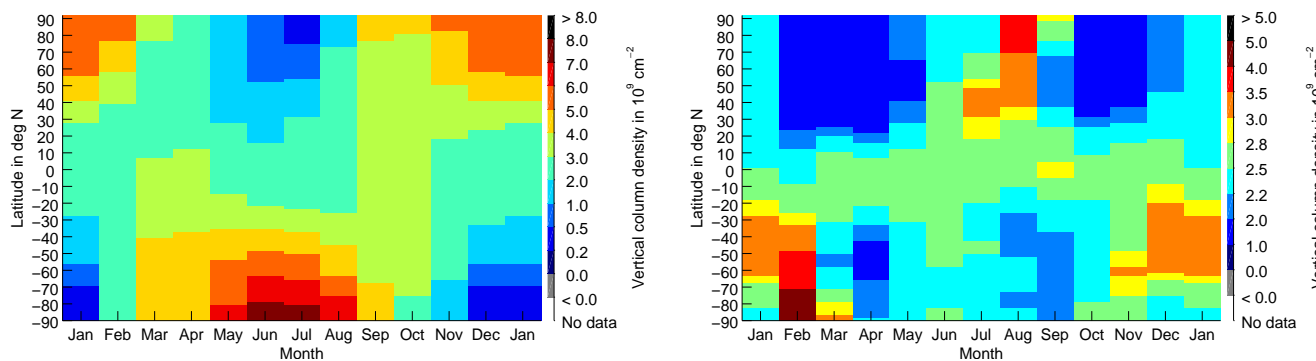
Figure 16. WACCM VCD timelines for different latitudes for Mg (left) and \text{Mg}^+ (right). Mg VCD varies between 0.5 \times 10^9 \text{ cm}^{-2} and 8 \times 10^9 \text{ cm}^{-2} and shows a clear seasonal cycle with a winter maximum, which is most pronounced at the poles. \text{Mg}^+ VCD varies from 1 \times 10^9 \text{ cm}^{-2} to 5 \times 10^9 \text{ cm}^{-2} , with most VCD values between 2 \times 10^9 \text{ cm}^{-2} and 3 \times 10^9 \text{ cm}^{-2} . A clear seasonal cycle with a summer maximum for \text{Mg}^+ is observed. SCIAMACHY results of VCD are shown in Figs. 5 and 9.
