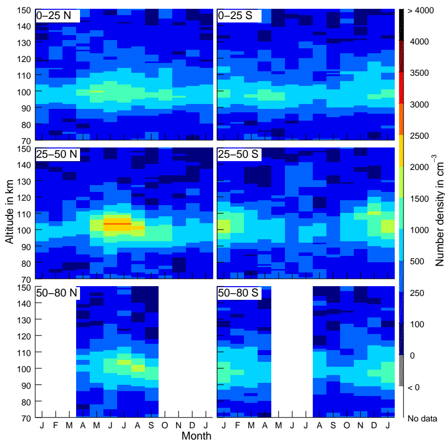
Figure 8. Seasonal variation of the vertical profile of \text{Mg}^+ (280.4 nm line) for different latitudinal zones (left: NH, right: SH, top: low latitudes, middle: mid latitudes, bottom: high latitudes), averaged over all available observations in 2008–2012. For all these latitudinal zones a seasonal cycle in the peak altitude with a summer maximum and a winter minimum can be observed. The seasonal variations are similar or larger than the month-to-month variations. The maximum peak altitude is 5–10 km higher than the minimum peak altitude. For mid latitudes, the peak altitude in the winter hemisphere is still higher than the peak altitude at the equator (see also Fig. 6).
