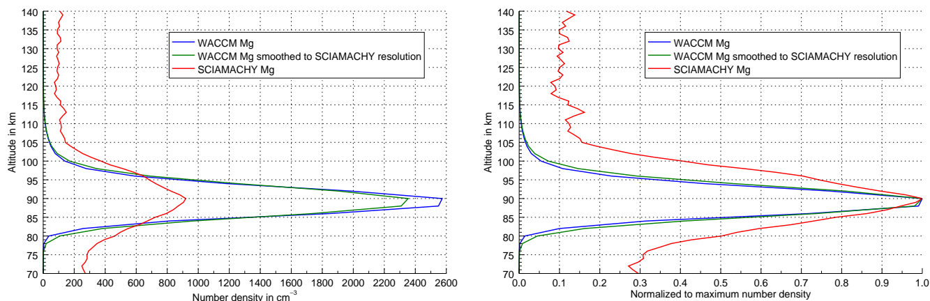
Figure 19. Equatorial annual mean vertical profile of Mg for SCIAMACHY and WACCM. The right plot shows the profiles normalized to the maximum of each profile, to better compare the shape of the profiles. The smoothed profile is smoothed with a triangular function with a base width of 4 km. The VCD between 70 and 140 km is 2.3 \times 10^9 \text{ cm}^{-2} for SCIAMACHY and 2.5 \times 10^9 \text{ cm}^{-2} for WACCM. Note that the statistical error for SCIAMACHY estimated by Langowski et al. (2013) (Fig. 21) is \approx \pm 200 \text{ cm}^{-3} for the low-density region above 100 km and below 80 km and \approx \pm 400 \text{ cm}^{-3} at 90 km.
