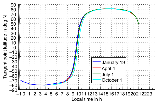
Figure 1. Local time at the tangent point of SCIAMACHY limb measurements at different latitudes for different seasons of the year.
