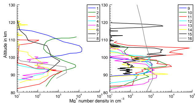
Figure 11. Measurements of the vertical \text{Mg}^+ number density profile mentioned in the text and listed in Table 1. Note that the data points are redrawn from the original figures, and not all details of the original figures may be captured.
