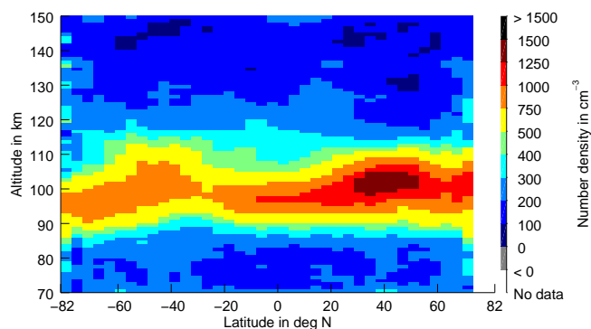
Figure 7. Latitudinal variation of \text{Mg}^+ profiles averaged over all available data for 2008–2012 for the \text{Mg}^+ line at 280.4 nm.
