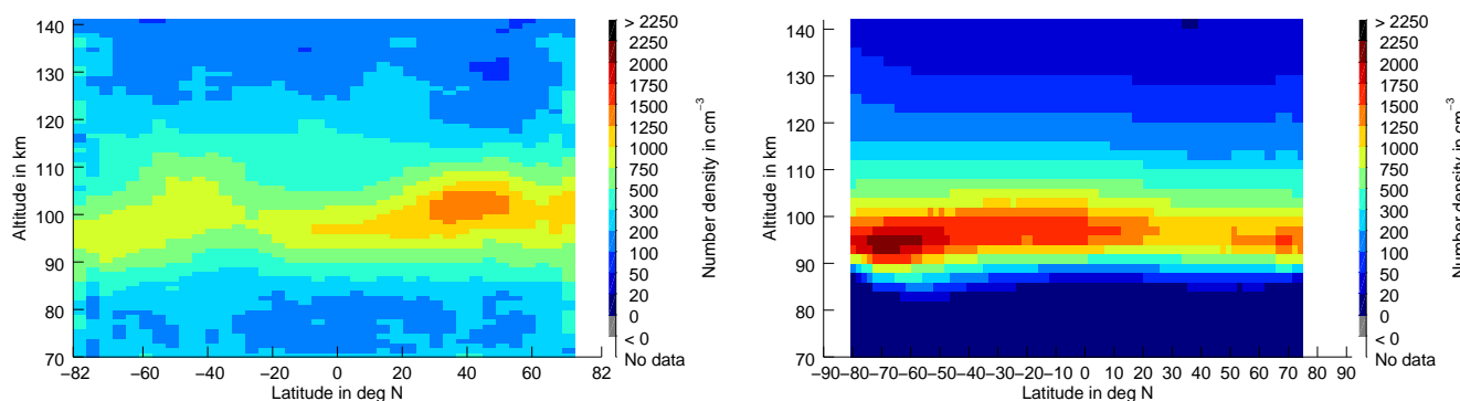
Figure 18. Annual means of \text{Mg}^+ for SCIAMACHY (left, 280.4 nm) and WACCM (right). SCIAMACHY shows a wider vertical profile, and a stronger latitudinal dependence of the peak altitude. The peak density of both is in very good agreement. The averaging for WACCM simulations is restricted to match the time periods, where SCIAMACHY measurements are available.
