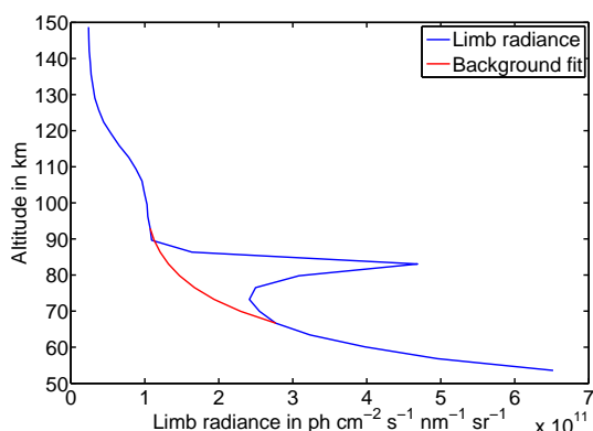
Figure 23. Averaged SCIAMACHY limb MLT signal between 458 and 552 nm showing a NLC signature at 84 km and a background fit. The NLC radiance is quantified as the summed up differences between the signal and the background fit in the vicinity of the NLCs signal.
