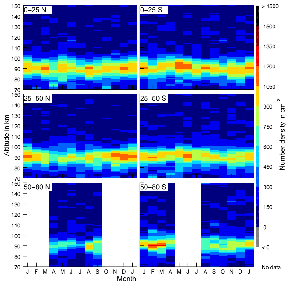
Figure 4. Seasonal variation of the vertical Mg profile for different latitudinal zones (left: Northern Hemisphere (NH), right: Southern Hemisphere SH, top: low latitudes, middle: mid latitudes, bottom: high latitudes). The peak altitude is at 90 km for all latitudes with variations of \pm 5 km. The month-to-month variations in peak altitude and density are bigger than any seasonal variations.
