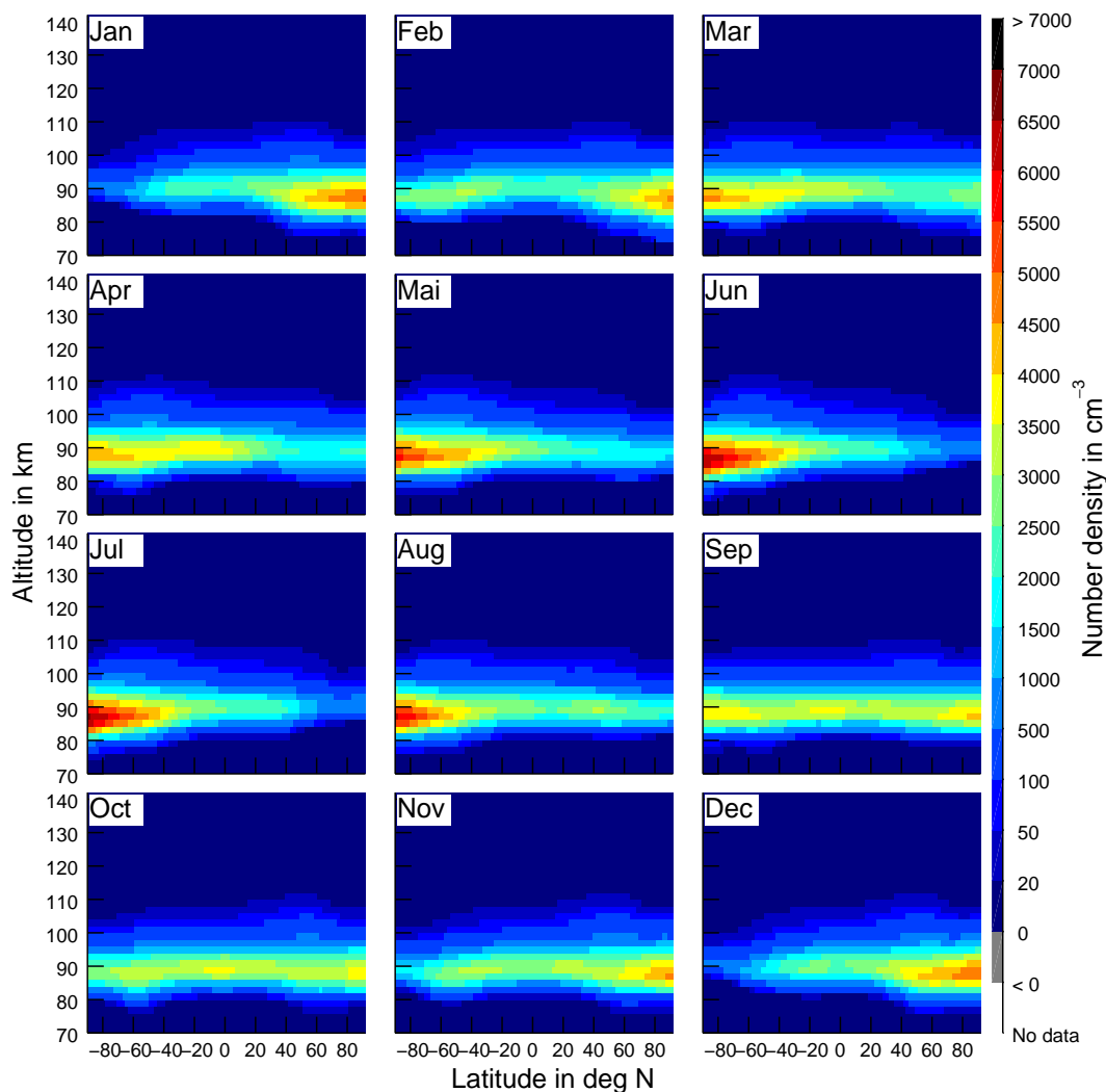
Figure 14. Monthly mean WACCM results for Mg averaged over 7 yr from 2005 to 2011. The model results show a clear seasonal cycle with a winter maximum, most pronounced at high latitudes.
