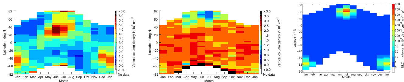
Figure 24. Vertical column density of \text{Mg}^+ (left), Mg (mid) and NLC radiance (right) retrieved from SCIAMACHY. A clear reduction of \text{Mg}^+ and Mg VCD is observed in the vicinity of NLCs. However, this is also observed in neighbouring regions without NLCs and can also be explained by other processes. (Note that the NLCs retrieval includes more latitudes from the ascending node side).
