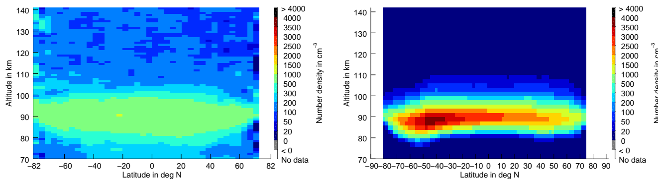
Figure 17. Annual means of Mg for SCIAMACHY (left) and WACCM (right). SCIAMACHY measures smaller peak density having a wider vertical profile than WACCM. The averaging for WACCM simulations is restricted to match the time periods, where SCIAMACHY measurements are available.
