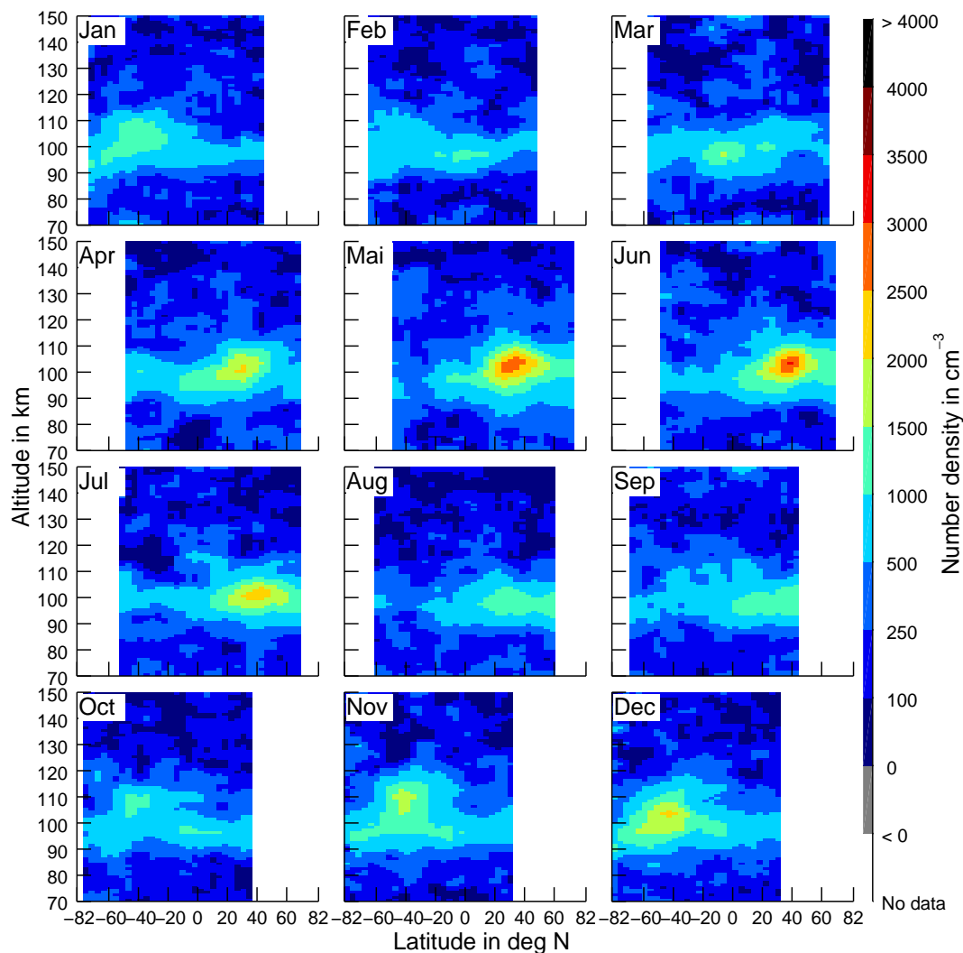
Figure 6. Latitudinal variation of monthly and zonally averaged \text{Mg}^+ profiles (for the years 2008–2012) retrieved from the \text{Mg}^+ line at 280.4 nm. \text{Mg}^+ shows a seasonal cycle with a summer maximum, which is especially pronounced in the region between 25° and 45° latitude in the summer hemisphere. Furthermore, in this region the peak altitude is about 105 km, which is up to 10 km higher than at the equator or at the poles.
