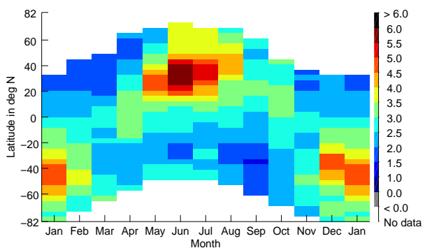
Figure 9. Seasonal variation of the \text{Mg}^+ vertical column density (VCD) between 70 km and 150 km and for different latitudinal regions, retrieved from the 280.4 nm line. A clear seasonal cycle with a summer maximum can be observed. The summer maximum in the NH has higher values compared to the one in the SH. The highest variability can be found between 25° and 50° in both hemispheres.
