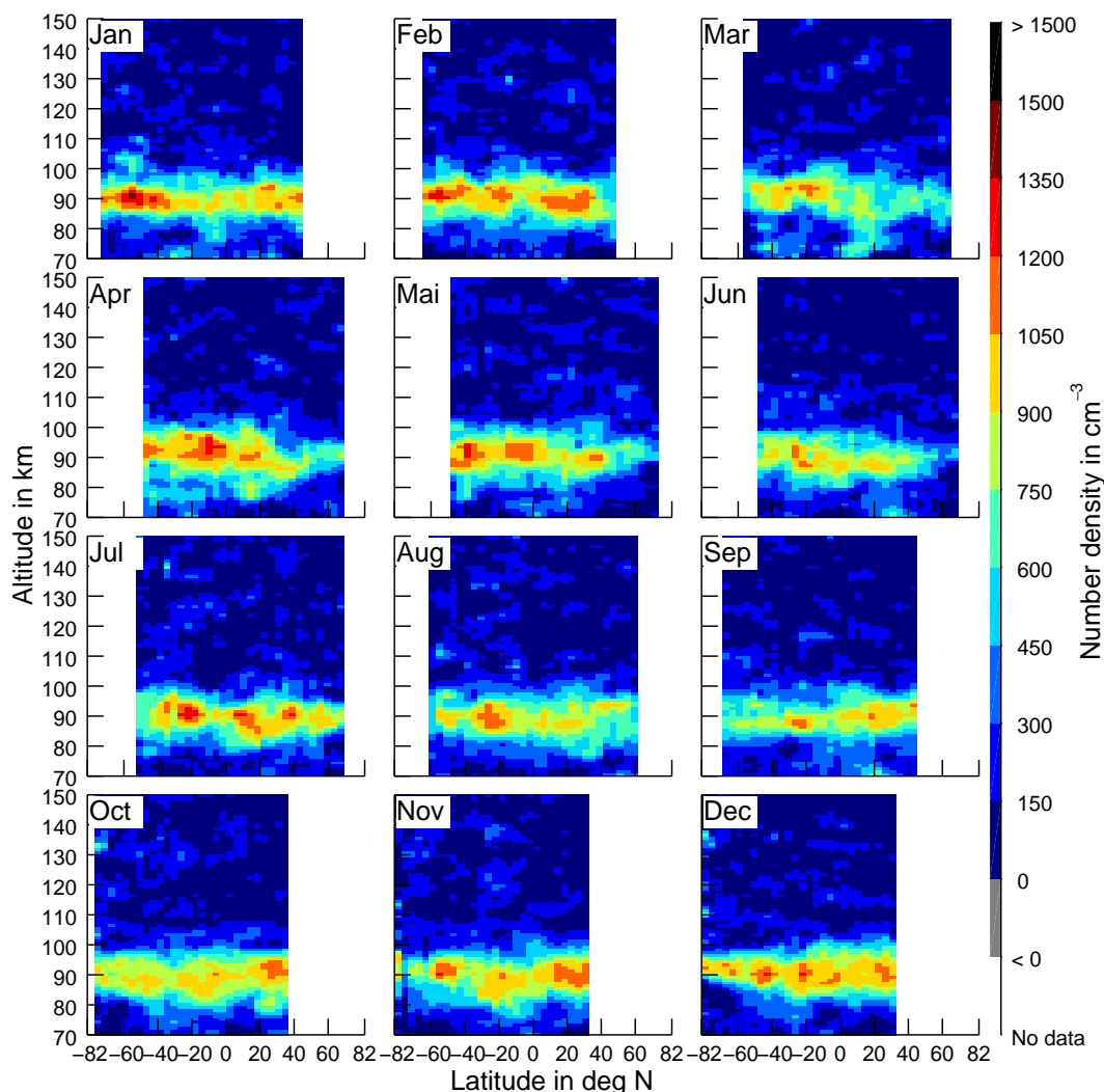
Figure 2. Latitudinal variation of monthly (averaged over all January, February, etc. results from 2008–2012) and zonally averaged Mg density profiles retrieved from the 285.2 nm line. The Mg layer peaks at around 90 km altitude and has a FWHM of about 15 km.
