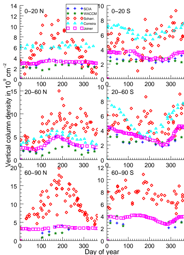
Figure 12. \text{Mg}^+ VCD results for different latitudinal regions and from different sources. The left column shows the NH and the right column the SH. From top to bottom results for low, mid and high latitudes are shown. Note that different sources originally used different time periods. The data used are from SCIAMACHY (blue) and WACCM (green) from this work (0–20° N/S, 20–60° N/S, 60–90° N/S, WACCM data co-located to SCIAMACHY coverage), from (Scharringhausen, 2007) (Figs. 7.3 and 7.4, red), from (Correira et al., 2008) (Fig. 1, cyan) and (Joiner and Aikin, 1996) (Figs. 10 and 11, magenta).
