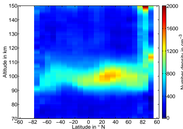
Figure 21. \text{Mg}^+ profiles averaged over all available data for 2008–2012 for the \text{Mg}^+ line at 280.4 nm. The stray-light contaminated measurements at the start of the sunlit part of each orbit are also used here extending the coverage to higher northern latitudes and even the ascending node side. High \text{Mg}^+ density is observed at the north pole. See Fig. 1 and Sect. 4 (second paragraph) for an explanation of the x -axis labels. Note that this is an older plot, which shows data with a wrong polarization correction, which is, however, unimportant for the effect shown here.
