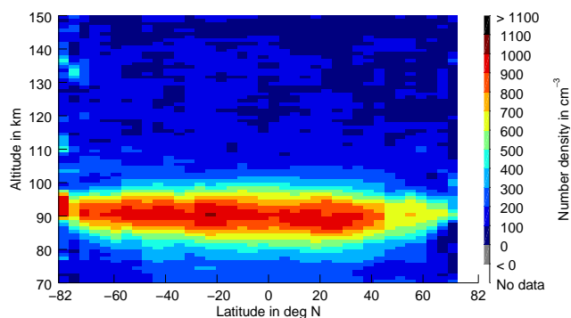
Figure 3. Latitudinal variation of Mg profiles averaged over all available data for the years 2008–2012. Note that only between 45° N and S do measurements from all 12 months contribute to the averages, while for high latitudes there is only summer coverage and/or near-terminator measurements.
