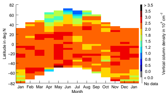
Figure 5. Seasonal variation of the Mg vertical column density (VCD) between 70 km and 150 km for different latitudinal regions. The VCD varies between 0.5 \times 10^9 \text{ cm}^{-2} and 3.5 \times 10^9 \text{ cm}^{-2} . No clear seasonal cycle is observed. Variations between consecutive days with measurements (at least 14 days difference) are even higher than the inter-monthly variations.
