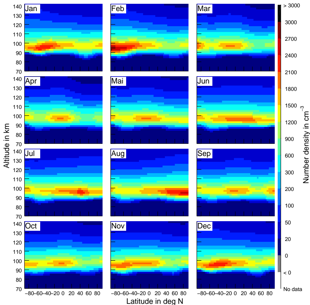
Figure 15. Monthly mean WACCM results for \text{Mg}^+ averaged over 7 yr from 2005 to 2011. The model results show a clear seasonal cycle with a summer maximum, most pronounced at high latitudes. There is also a second smaller maximum at high latitudes for the winter hemisphere.
