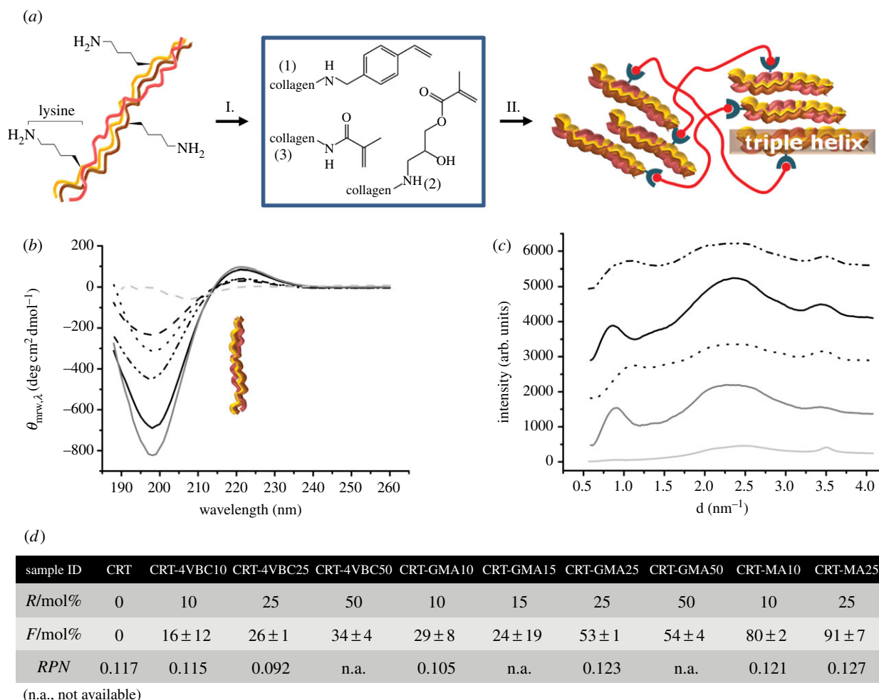
Figure 1. (a) Collagen lysines are covalently functionalized with vinyl moieties, i.e. 4VBC (1), GMA (2) and MA (3), respectively (I); UV irradiation leads to the formation of a covalent hydrogel network (II). (b) CD spectra of samples: gelatin (light grey dashed line), CRT (grey solid line), CRT-MA10 (black dotted line), CRT-MA25 (black dashed line), CRTGMA25 (black solid line), CRT-4VBC25 (black double dot-dashed line). The 221 nm peak is clearly detected in all collagen spectra, revealing the presence of triple helices in functionalized precursors. (c) WAXS spectra of samples: gelatin (light grey dashed line), CRT (grey solid line), CRT-MA10* (black dotted line), CRT-GMA50* (black solid line) and CRT-4VBC25* (black double dotted-dashed line). The WAXS peak ( d \sim 1.1 nm; 2\theta \sim 8^\circ ) related to molecular packing of collagen can still be observed in photo-activated systems, resulting in at least 70% retention of native collagen triple helices. (d) Molar excess of monomer with respect to collagen lysines ( R ), degree of collagen functionalization ( F ) and CD ratio ( RPN ) between positive and negative magnitudes are provided for each functionalized collagen formulation. (Online version in colour.)
