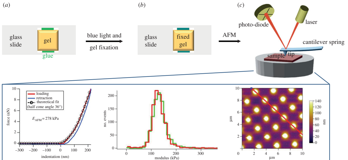
Figure 3. Sample preparation for AFM. (a) A microscope glass slide is coated with a photo-curable adhesive above which the collagen hydrogel is laid. (b) Blue light is applied to the slide so that the hydrogel is fixed. (c) The hydrogel-bearing slide is analysed via AFM. Bottom (from left to right): exemplary AFM force-indentation curve deriving from conical indentation on hydrogel CRT-MA10 * ; elastic modulus distributions obtained with 3 nN indentation force in two different regions of hydrogel CRT-MA10 * ; AFM image of a standard tip calibration grid with an array of sharp conical spikes. (Online version in colour.)
