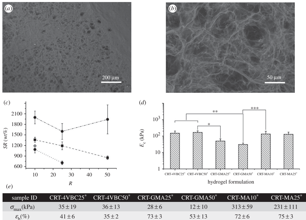
Figure 2. Exemplary SEM images of collagen hydrogel (CRT-GMA50*) following network equilibration in 25°C distilled water ( a : \times 100 , b : \times 1000 ). ( c ) SR of collagen hydrogels synthesized with varied molar excess of monomer with respect to lysine content ( R ) and incubated in distilled water. Dashed-dotted line, CRT-4VBC*; dashed line with squares, CRT-GMA*; dotted lines with circles, CRT-MA*. Swelling of hydrogel CRT-MA10* (grey diamond) was exemplarily measured in PBS instead of distilled water. ( d ) Compressive moduli ( E_c ) of collagen hydrogels; *, ** and *** indicate that E_c means of corresponding samples are significantly different (at the 0.05 level, Bonferroni test). ( e ) Maximal stress ( \sigma_{\max} ) and compression at break ( \epsilon_b ) measured during hydrogel compression.
