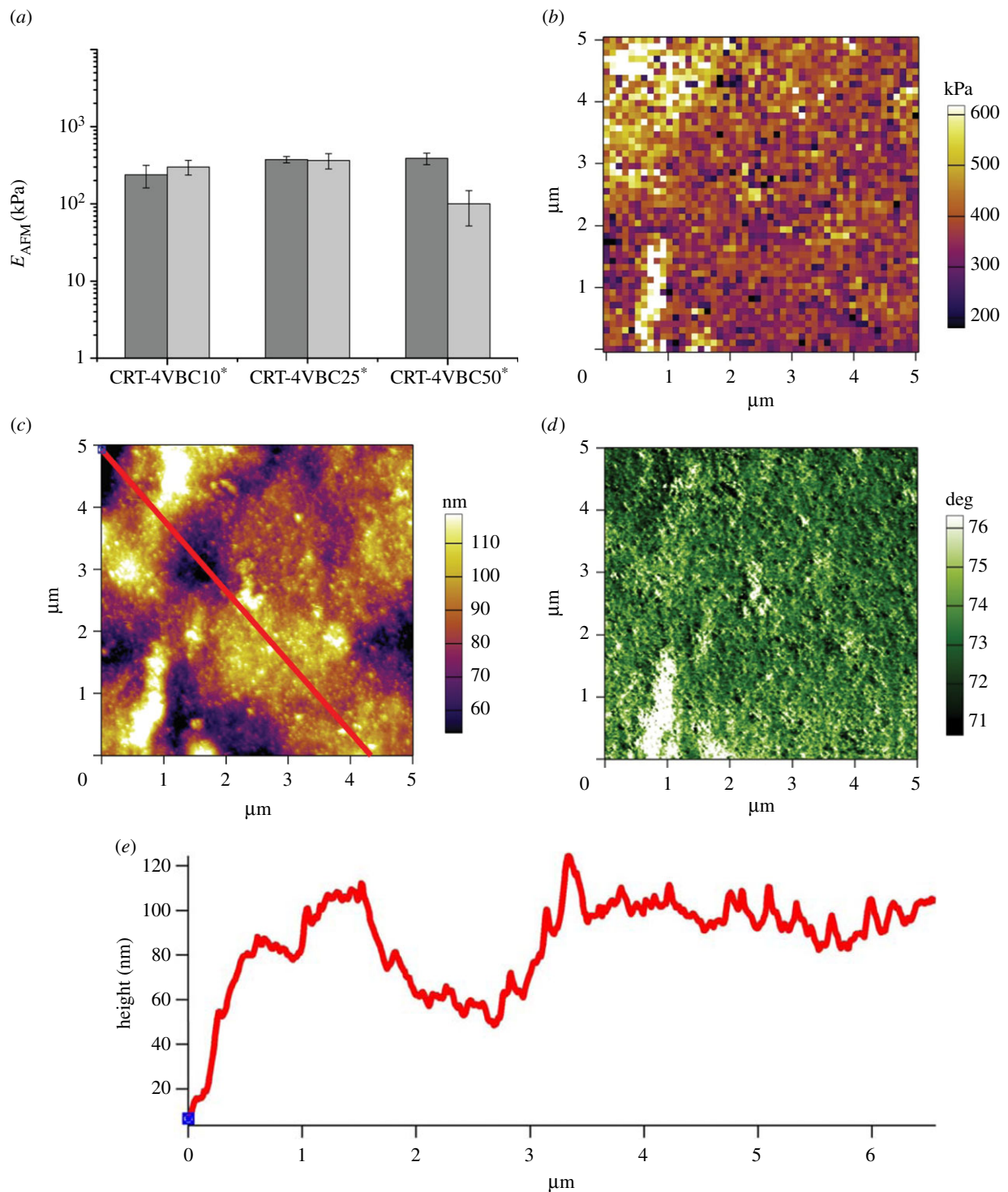
Figure 4. (a) Variation of E_{AFM} in hydrogels CRT-4VBC* determined via AFM indentation. Two replicates were used for sample CRT-4VBC10*, while two different regions in the same replica were investigated for the other two sample formulations. (b–d) Exemplary E_{AFM} map (b, 5 nN indentation force), surface image (c) and phase tapping mode image (d) obtained in hydrogel CRT-4VBC50*. As expected, no collagen fibrils could be observed on the material surface, since these hydrogels were prepared in 10 mM HCl solution, with which no fibrillogenesis can occur. (e) Height profile determined along the cross line section of figure 2c. (Online version in colour.)
