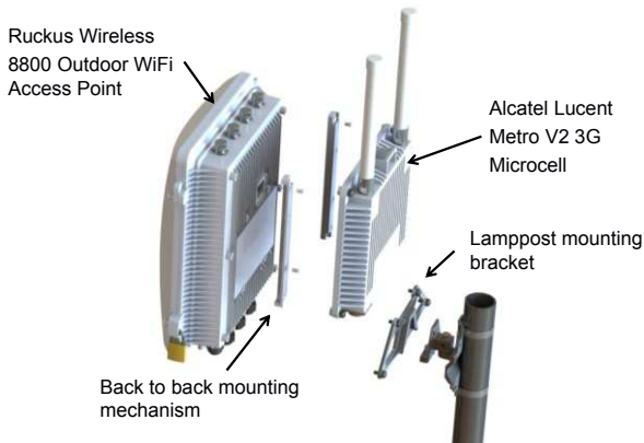
Fig. 2. Exploded schematic of the Telefonica 3G/Wi-Fi microcell.
