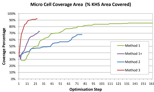
Fig. 7. Percentage of the KHS high traffic area covered versus the optimisation steps taken to achieve these coverage levels for the four SON methods considered.
