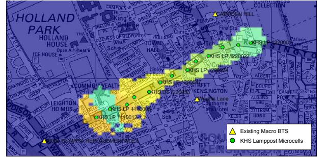
Fig. 5. KHS microcell best server coverage areas delivered by Method 1+.
