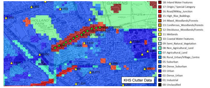
Fig. 3. Clutter Categories for Kensington small cell simulation area — showing the use of clutter category 17 to define the KHS high traffic area surrounding the thirteen lamppost microcells.
