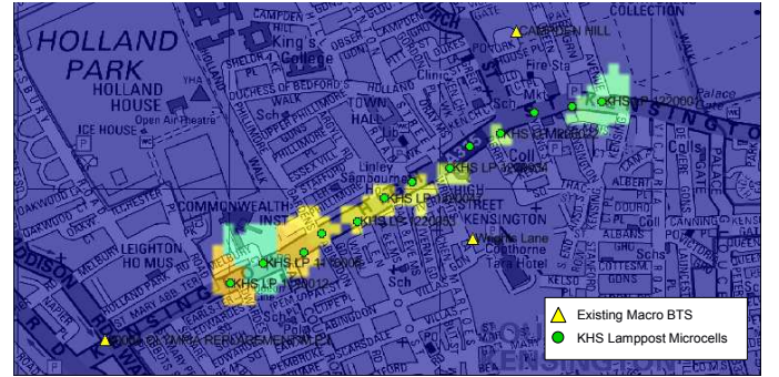
Fig. 4. KHS Lamppost microcell best server areas prior to network optimisation. Microcell BTS maximum output power = +10dBm.
