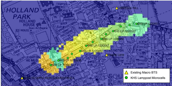
Fig. 6. KHS microcell best server coverage areas delivered by Method 3.
