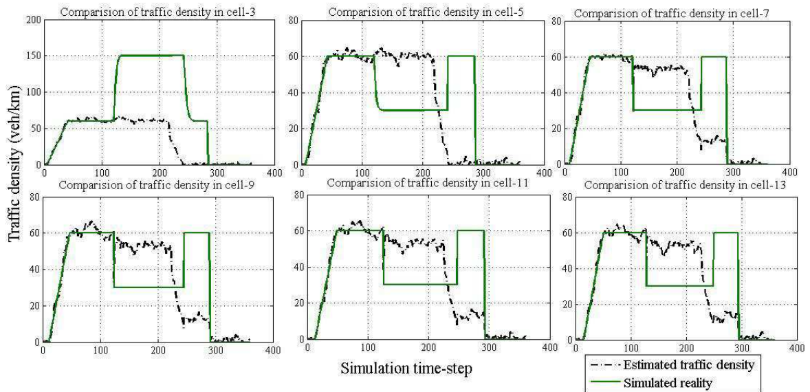
Fig.5. Comparison of estimated traffic density with simulated reality
