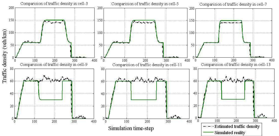
Fig.4. Comparison of estimated traffic density in cells 3, 5, 7, 9, 11 and 13 with simulated reality
