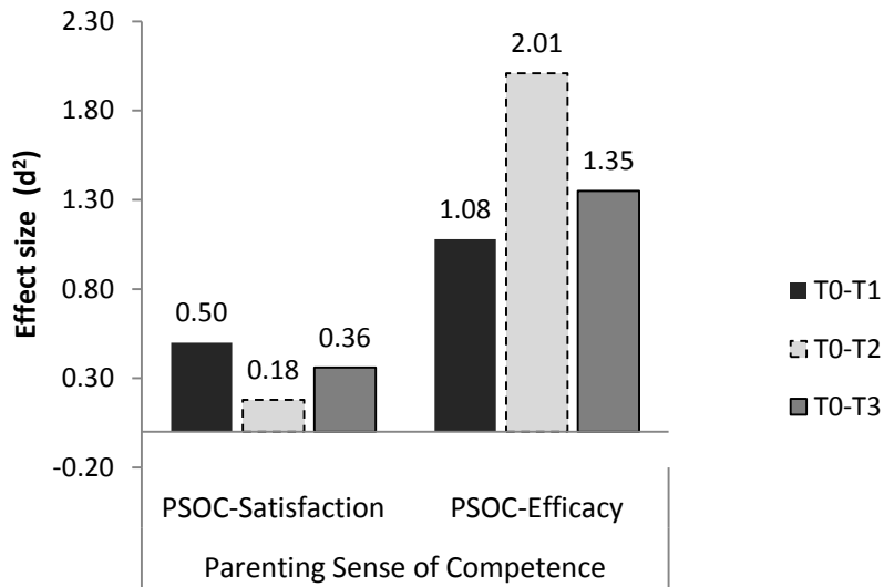
Figure 3. Effect sizes for PSOC-Satisfaction and PSOC-Efficacy subscales
