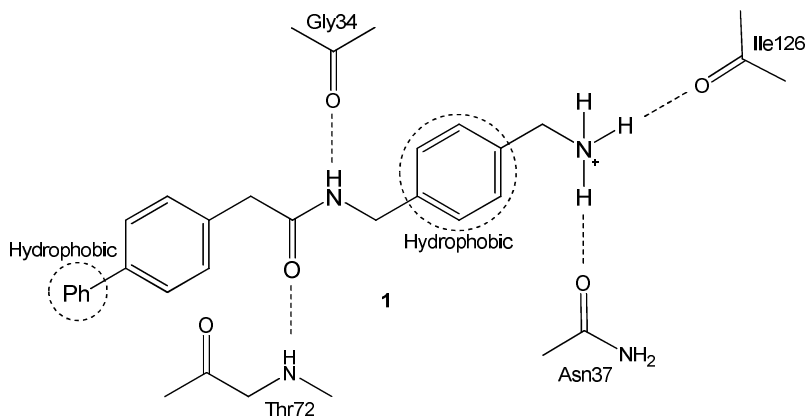
Figure 2. Schematic showing the proposed interactions of inhibitor 1 (shown in ionic form) with BACE1.
