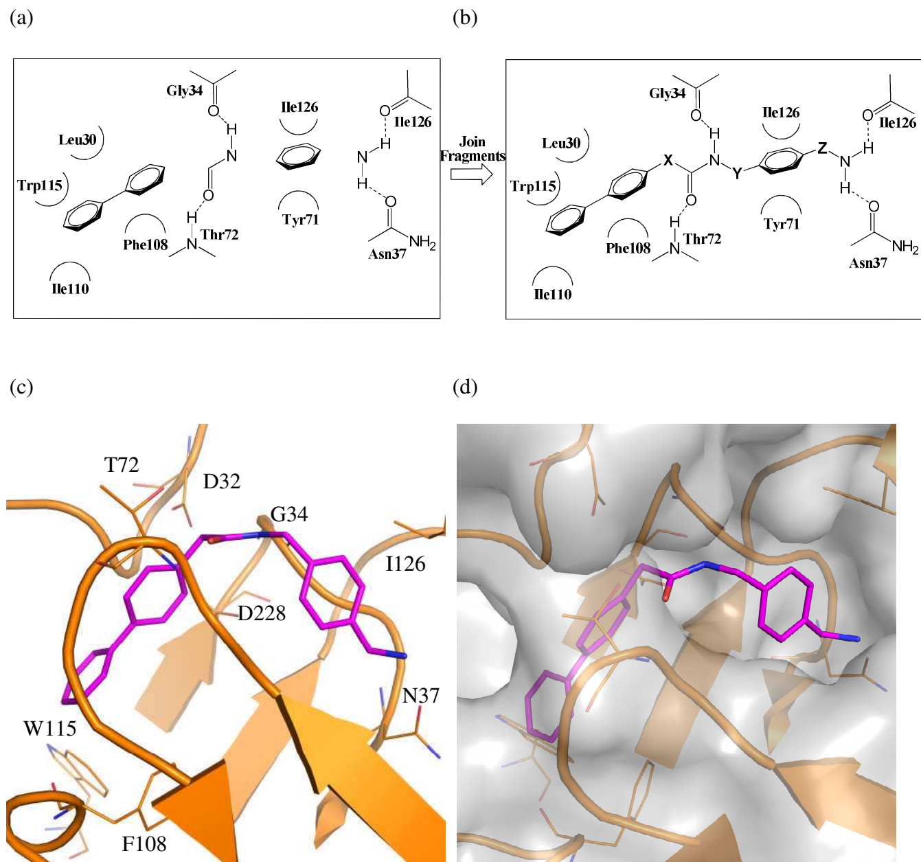
Figure 1. De novo design of biphenylacetamide inhibitor 1 in the BACE1 binding pocket (PDB 1M4H). (a) Fragments docked into selected individual target sites, (b) fragments joined to yield complete ligand scaffold, (c) proposed binding mode of 1 (magenta) with key residues labeled (orange); and (d) proposed binding mode of 1 with surface of the binding pocket.
