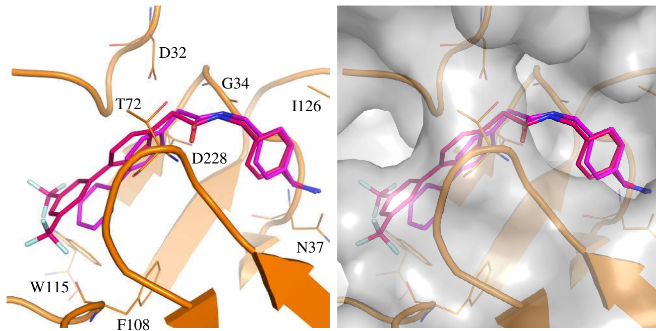
Figure 3. The optimized candidate structure 14 (pink), designed using SPROUT-HitOpt, overlaid with the predicted binding pose of 1 (magenta). (a) Proposed binding mode of 14 (pink) with key residues labeled (orange); and (b) proposed binding mode of 14 with surface of the binding pocket.
