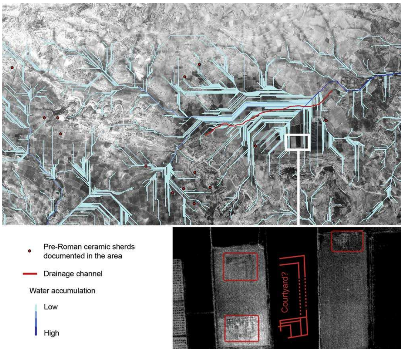
Fig. 3. Water accumulation and detail of buried structures at the Calabarra area.
