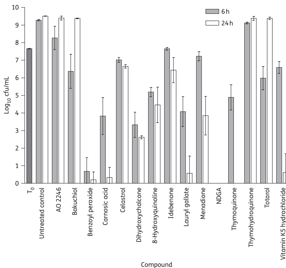
Figure 1. Evaluation of the bactericidal activity of redox-active compounds at 4× MIC for S. aureus SH1000. T 0 represents the number of cells present in cultures prior to addition of compounds. Results are means of at least three independent replicates and error bars show standard deviations.
