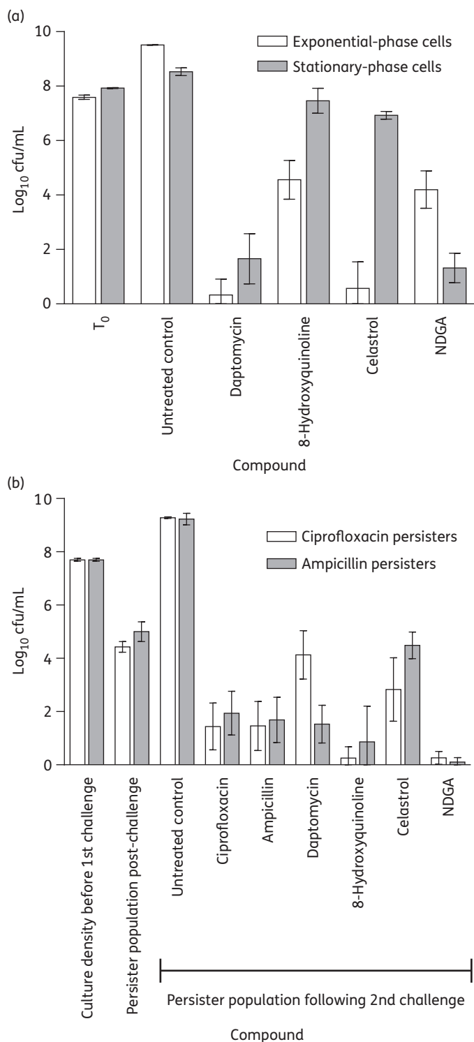
Figure 3. Viability of S. aureus SH1000 slow-growing and persister cells following exposure to compounds for 24 h. (a) Exponential- and stationary-phase cell viability following exposure to biofilm eradicator or biofilm non-eradicators at the MBEC or biofilm non-eradicators at 256 mg/L. T 0 is the culture density before the addition of compounds. (b) Cell viability of ciprofloxacin and ampicillin persisters following exposure to compounds at 10× MIC. Results are means of at least three independent determinations and error bars show standard deviations.
