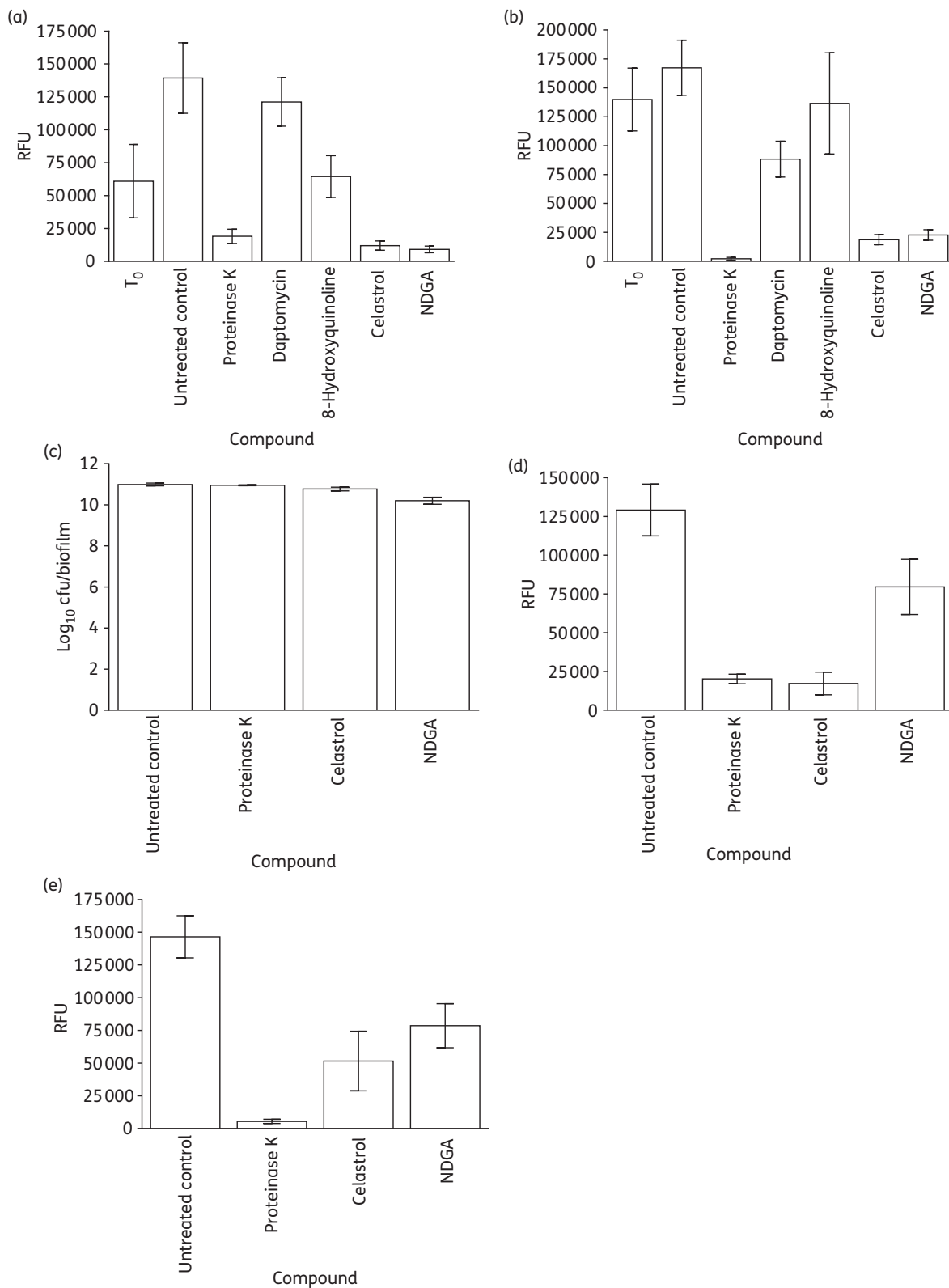
Figure 4. Cell viability and quantification of adherent material by fluorescent staining following exposure of biofilms to compounds at 256 mg/L for 24 h or 60 min. (a) Attached matrix (24 h). (b) Attached cells (24 h). (c) Total biofilm cell viability (60 min). (d) Attached matrix (60 min). (e) Attached cells (60 min). The data labelled T_0 show the quantity of matrix and cells before the addition of compounds and RFU denotes relative fluorescence units. Results are means of at least three independent determinations, with error bars showing standard deviations.
