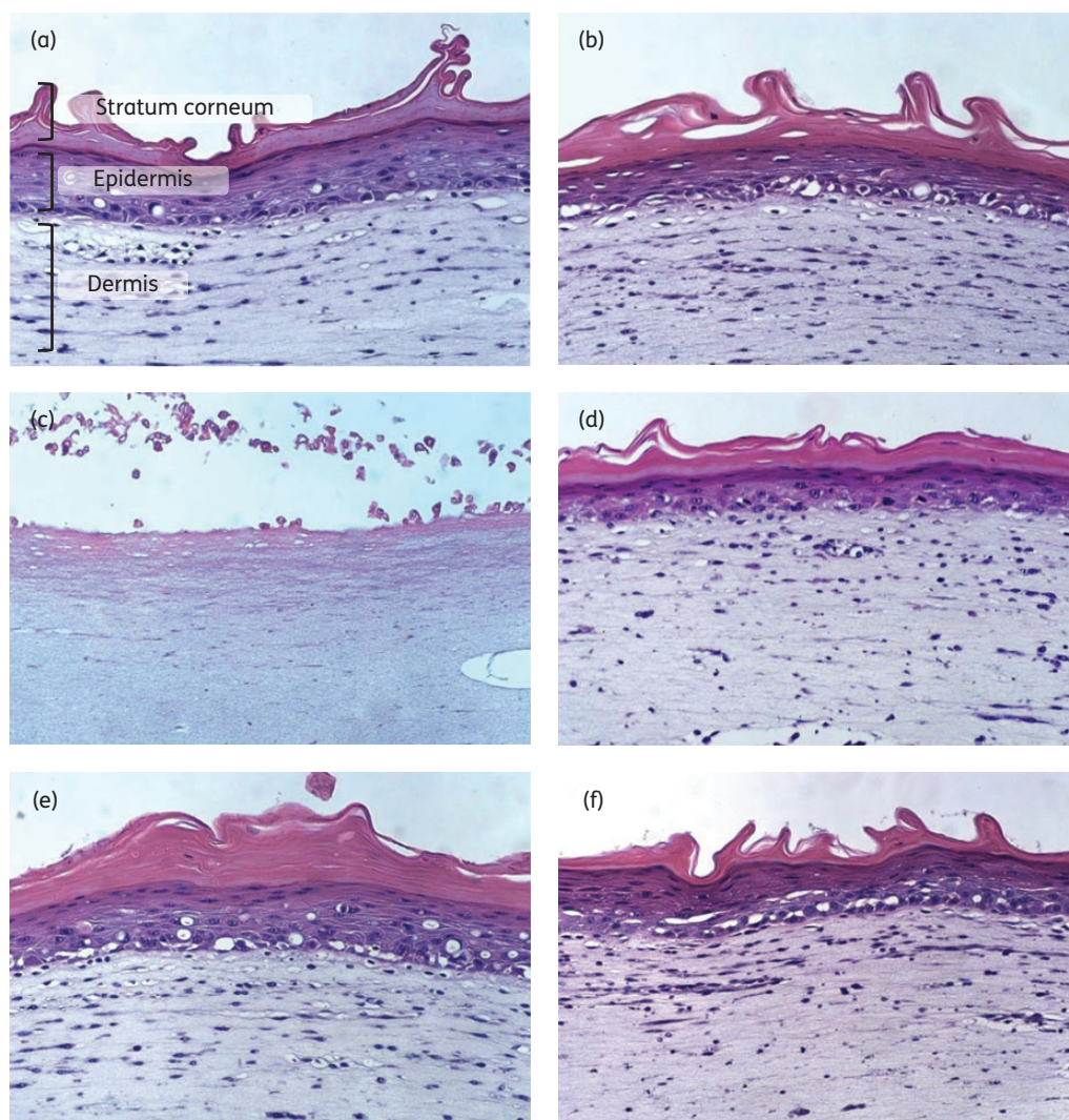
Figure 5. Haematoxylin/eosin-stained sections of LabSkin™ exposed to compounds for 24 h. (a) Untreated control. (b) Solvent (0.2% ethanol, v/v). (c) SDS (5%, w/v). (d) Mupirocin at 10× MIC (0.000125%, w/v). (e) Celastrol at 10× MIC (0.001%, w/v). (f) NDGA at 4× MIC (0.0256%, w/v).
