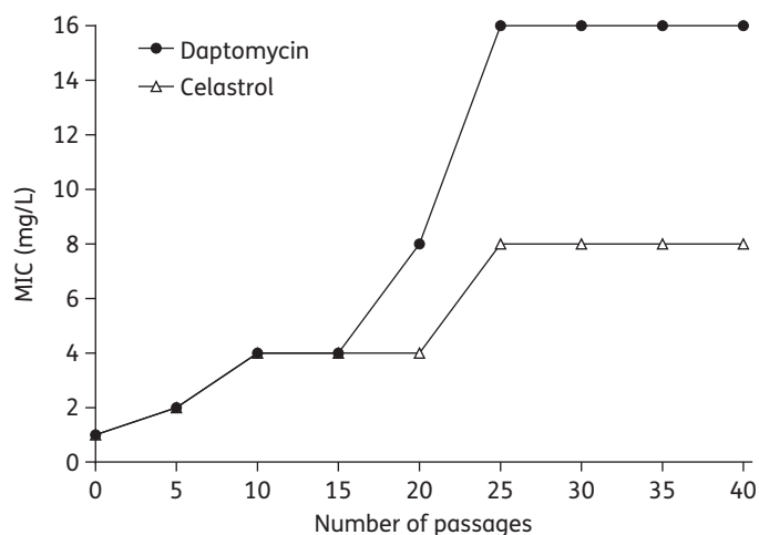
Figure 6. Selection of daptomycin- and celastrol-resistant mutants of S. aureus SH1000. Results are representative of experiments carried out on eight independent occasions using the extended gradient MIC method. 23
