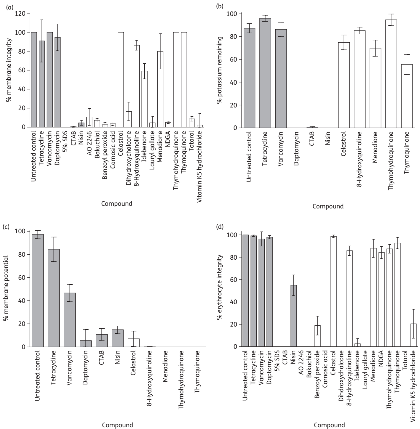
Figure 2. Effect of redox-active compounds and comparator agents at 4\times MIC on bacterial and mammalian membranes. Bacterial membrane integrity was measured using the BacLight TM assay (a) and by monitoring leakage of intracellular potassium (b). Bacterial membrane potential was measured by leakage of DiSC 3 (5) (c). Mammalian membrane integrity was measured by leakage of haemoglobin from erythrocytes (d). Filled bars show comparator agents. Results are means of at least three independent determinations and error bars show standard deviations.
