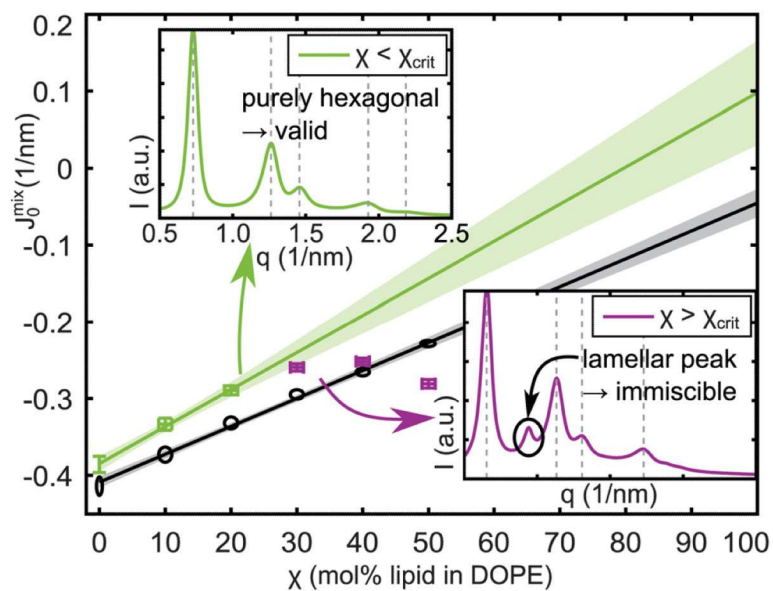
Fig. 2. Determination of J_0^{\text{DPPC}} at 25^\circ\text{C} (crosses) and J_0^{\text{POPC}} at 45^\circ\text{C} (ellipses) by extrapolation of J_0^{\text{mix}} towards \chi = 100\% . The insets show X-ray patterns for the last valid (top left) and the first immiscible DPPC data points (bottom right).
