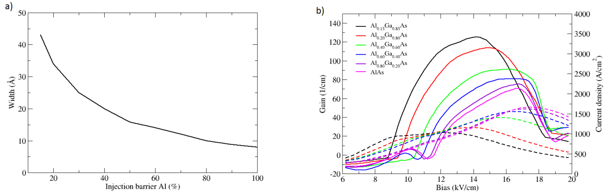
Figure 2: (a) Barrier width dependence on height to obtain injection coupling strength of \sim 2.9 meV. (b) Gain (solid) and current (dashed) versus applied bias for varying injection barrier alloy content at 4.2 K lattice temperature.
