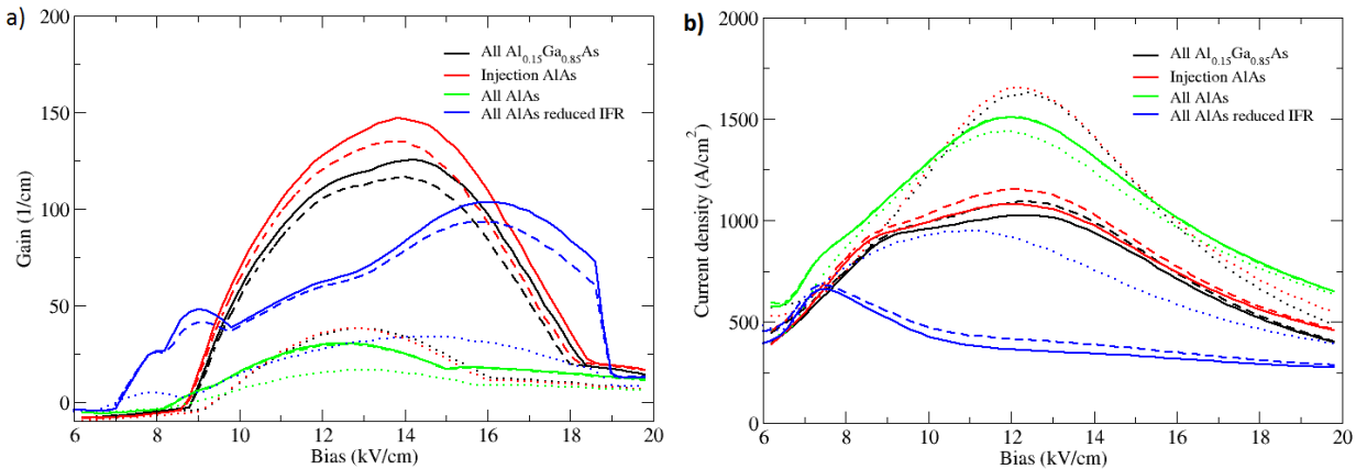
Figure 3: Gain (a) and current (b) versus applied bias for the reference structure [2], reference with AIAs injection barrier and all AIAs barrier structures [3] at 4.2 K (solid), 77 K (dashed) and 200 K (dotted) lattice temperatures.
