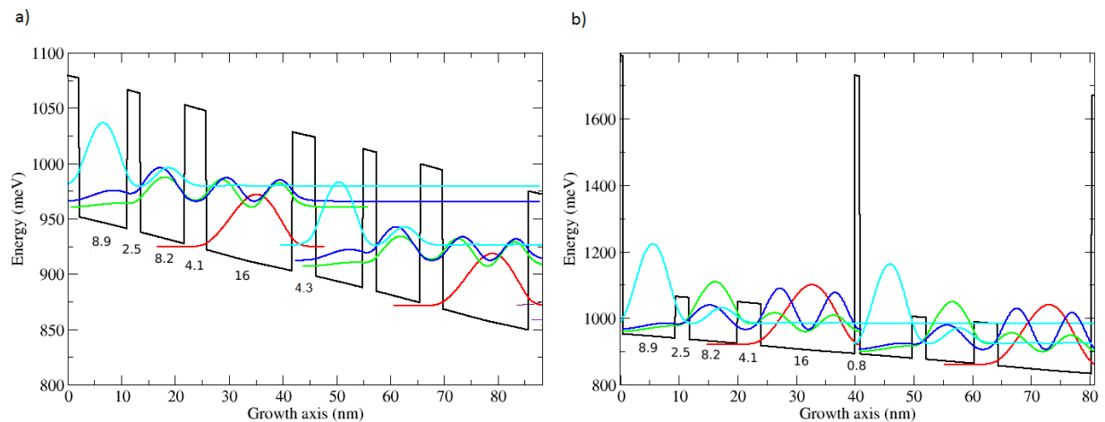
Figure 1: (a) Band diagram of the relevant wavefunctions for the current T = 200 K record design [2] at 12.2 kV/cm (b) structure with AIAs injection barrier width modified to obtain similar injection coupling of \sim 2.9 meV at 18 kV/cm.
