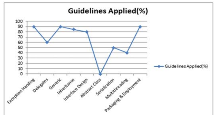
Figure 6. Represent the Component Design Guidelines in Percentage.
