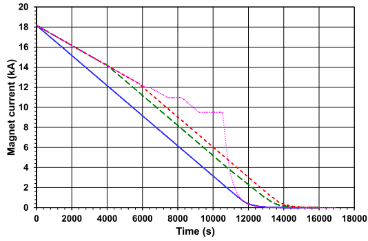
Fig. 2. CMS magnet current discharges from 18.2 to 0 kA made on July 17 and 18, 2015 (blue smooth line), September 21 and 22, 2015 (green dashed line), September 10, 2016 (red small dashed line), and November 30, 2017 (pink dotted line).
