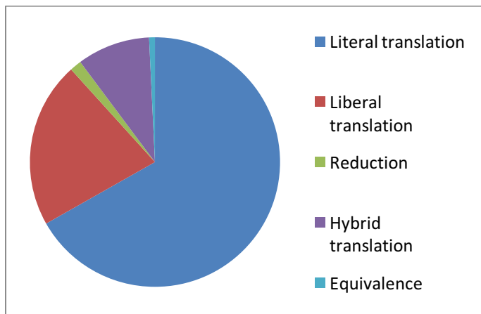
Figure 2: Translation techniques of indigenous concepts in The Governance of China
