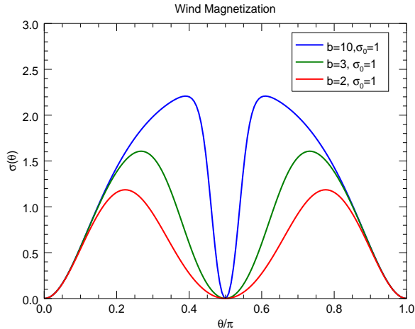
FIGURE 4. Shape of the wind magnetization \sigma(\theta) for the value of \sigma_0 = 1 employed in our 3D simulation and for three values of b . The upper (blue) curve is the case with a narrow striped wind region used here, with \sigma_{\text{eff}} = 1.5 , while the bottom (red) curve refers to a case that approximately reproduces the magnetization function as in the B3D run in Porth et al. (2014b).
