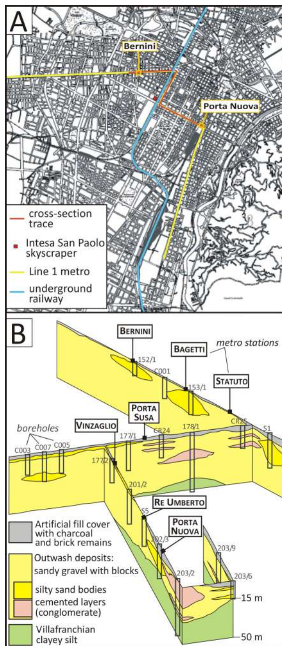
Fig. 15 - A) Main recent excavations in the subsoil of Turin: 1) subway (Line 1 of the Metro, 15 km); 2) underground railway pass (12 km); 3) Intesa Sanpaolo skyscraper. B) Cross section along the subway involving the variously cemented Dora Riparia River outwash sediments (modified from a Geodata sketch).
