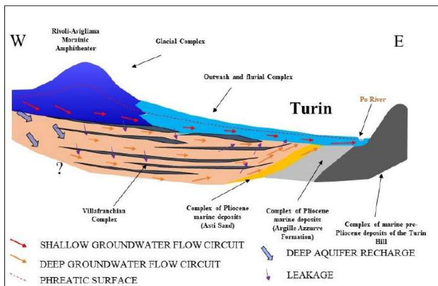
Fig. 21 - Conceptual hydrogeological model of the Turin area, showing deep aquifers, conditioned by the buried hilly structure, and a surficial aquifer both flowing from the Alps towards east.
