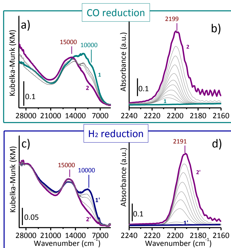
Figure 2: Part a) DR UV-Vis-NIR spectra in the d-d region of the CO-reduced 0.5Cr/Al 2 O 3 catalyst (spectrum 1), and of the same sample in the presence of CO ( P_{CO} = 100 mbar) at room temperature (spectrum 2). Grey spectra show the effect of gradual CO desorption at room temperature. Part b) Evolution of the FT-IR spectra (magnification of the \nu(\text{CO}) region) upon CO adsorption at room temperature on the CO-reduced 1.0Cr/Al 2 O 3 catalyst as a function of P_{CO} coverage, from P_{CO} = 100 mbar (spectrum 2) to zero (spectrum 1). Parts b) and d): as part a) and c) for H 2 -reduced 0.5Cr/Al 2 O 3 and 1.0Cr/Al 2 O 3 , respectively.
