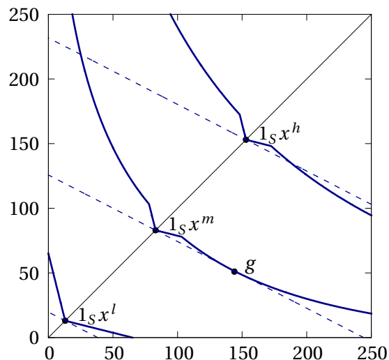
Figure 3: \bigcap_i C_i(1_S x_i) \neq \emptyset is not sufficient for risk sharing.
