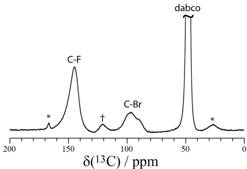
Figure S4. Experimental ^{13}\text{C} solid-state NMR spectrum of 5 ( p -DBrTFB)(dabco). The “dabco” label denotes the resonance assigned to dabco ( \delta(^{13}\text{C}) = 47.6 \pm 0.1 ppm), whereas the “C-Br” label denotes the resonance assigned to the carbon covalently bonded to bromine ( \delta(^{13}\text{C}) = 102.6 \pm 1.3 ppm to 85.3 \pm 2.1 ppm), and the “C-F” symbol denotes the carbon covalently bonded to fluorine ( \delta(^{13}\text{C}) = 102.6 \pm 1.3 ppm). The asterisks denote spinning sidebands. The dagger indicates a trace impurity.
