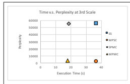
(g) Time v.s. perplexity at 3rd scale (NYSK dataset)
