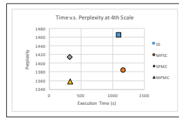
(b) Time v.s. perplexity at 4th scale (NIPS dataset)
