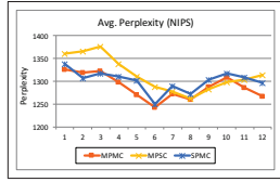
(c) Avg. perplexity over time (NIPS dataset)
