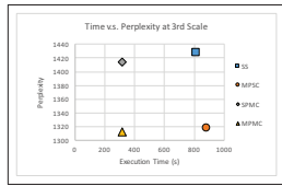
(a) Time v.s. perplexity at 3rd scale (NIPS dataset)
