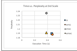
(d) Time v.s. perplexity at 3rd scale (Apple Stock dataset)
