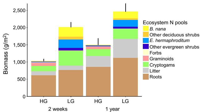
FIGURE 1 Above-ground and below-ground plant biomass, and plant litter ( \text{g}/\text{m}^2 ) in each ^{15}\text{N} -enriched plots at the heavily (HG) and lightly grazed (LG) sites at 2 weeks and 1 year after the addition of the labelled ^{15}\text{N} -urea within the system. Bars represent mean biomass for each ecosystem N pools and the error bars account for the standard error for the total biomass for each sites in each sampling year [Colour figure can be viewed at wileyonlinelibrary.com ]
