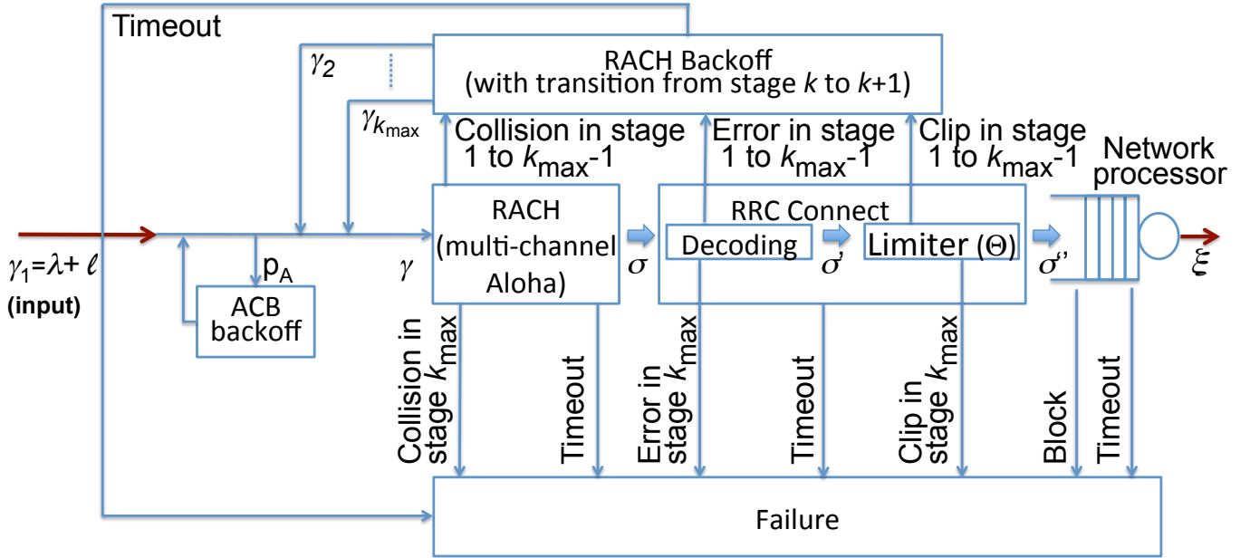
Fig. 2. Block diagram representing the system with primary and secondary flows accessing resources via RACH channels and RRC connect procedure. Flow \ell is subject to ACB and all accepted requests are served in FIFO order.
