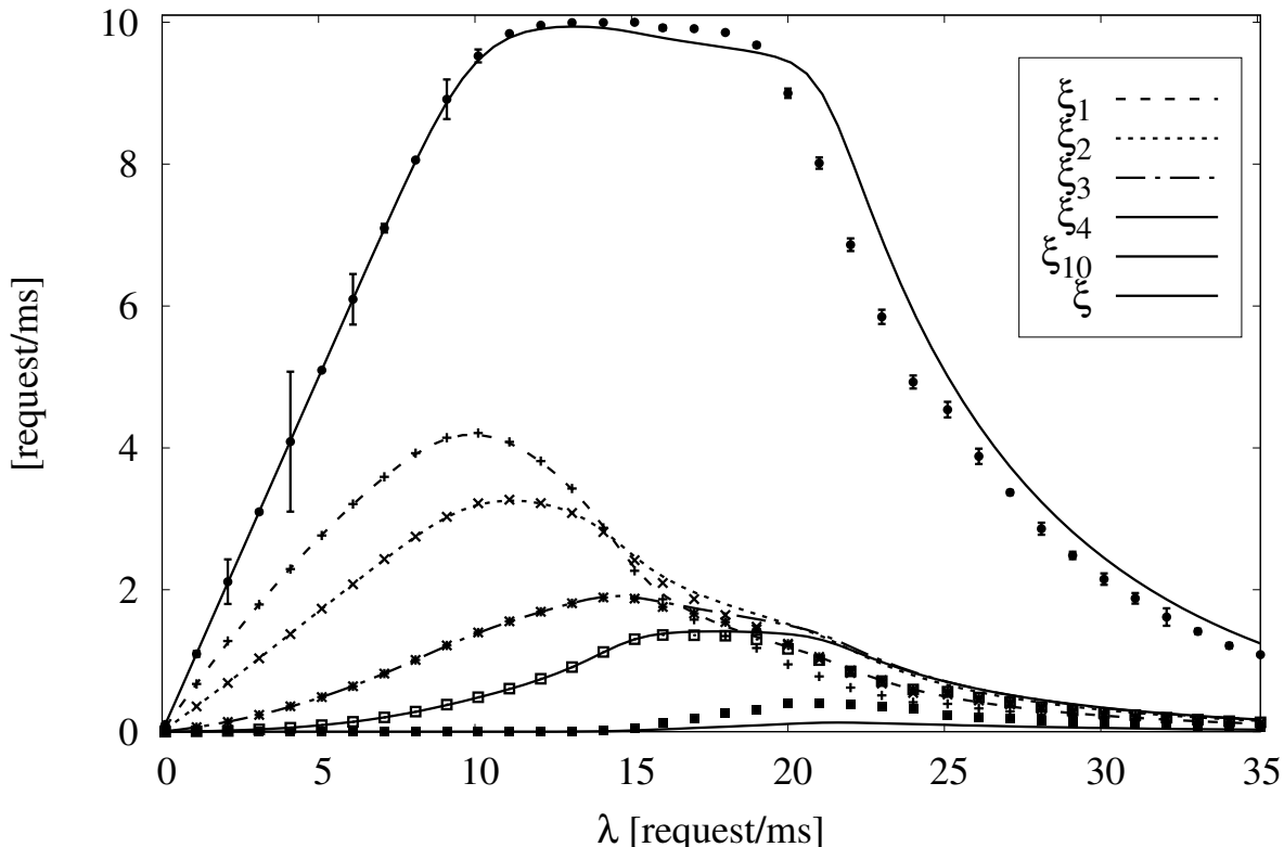
Fig. 6. Validation of the analytical model through simulation with primary flow only: network throughput \xi^{(\lambda)} and its per-stage components \xi_i^{(\lambda)} (for readability the figure only shows \xi^{(\lambda)} , \xi_1^{(\lambda)} , \xi_2^{(\lambda)} , \xi_3^{(\lambda)} , \xi_4^{(\lambda)} , and \xi_{10}^{(\lambda)} ).
