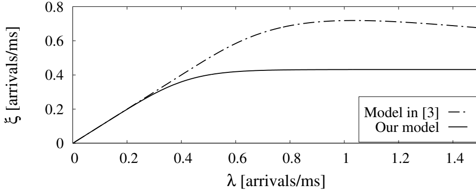
Fig. 3. Comparison between our simple model and the M2M model by Madueño et al. [3], which follows the behaviour of LTE-A signalling operations in detail. The latter is not meant to describe the behaviour of the system in saturated conditions, and hence a fair comparison with our model is possible only in the leftmost part of the figure.
