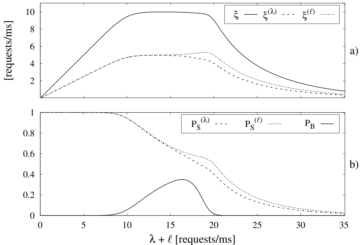
Fig. 10. Flows with different priorities: a) system throughput, b) P_S and P_B
