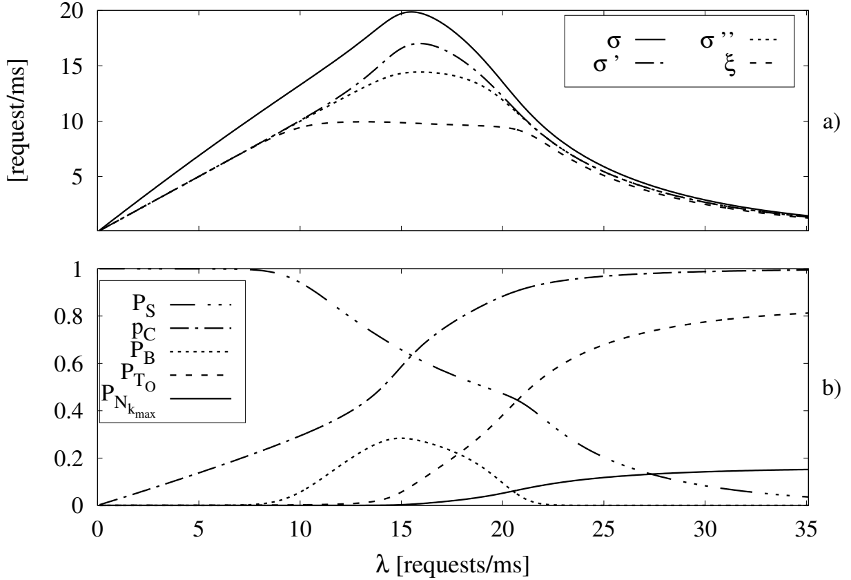
Fig. 5. System behaviour in the reference scenario in presence of flow \lambda : a) network throughput and flows leaving the RACH and the RRC connect phases with a success; b) stage probabilities.
