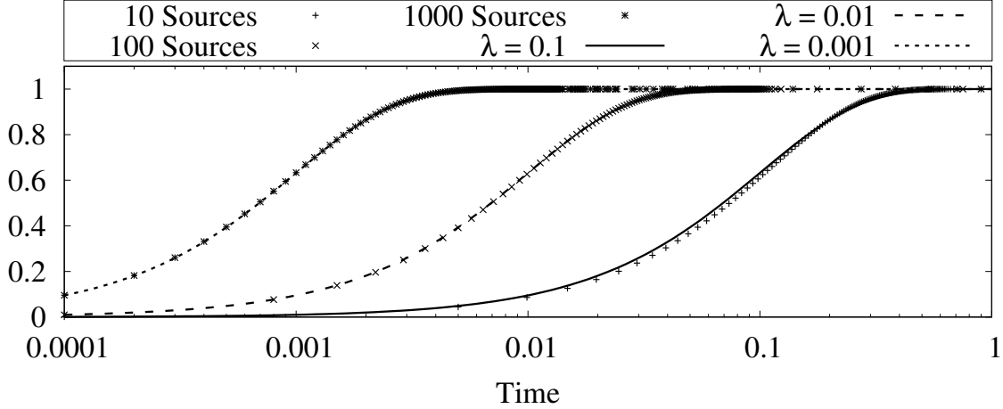
Fig. 4. Comparison of the CDF of a Poisson arrival stream against the one resulting from the superposition of 10, 100, 1000 arrival streams with interarrival times distributed according to a \mathcal{U}(0.9, 1.1) .
