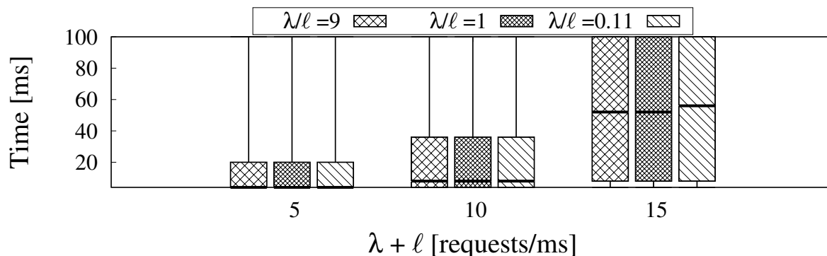
Fig. 11. Primary flow delay distribution in case of a success in the system with multiple flows
