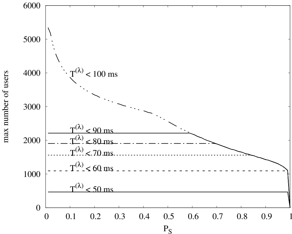
Fig. 9. Max number of MTDs that can be connected to a BS to guarantee success probability above a threshold and latency below a threshold
