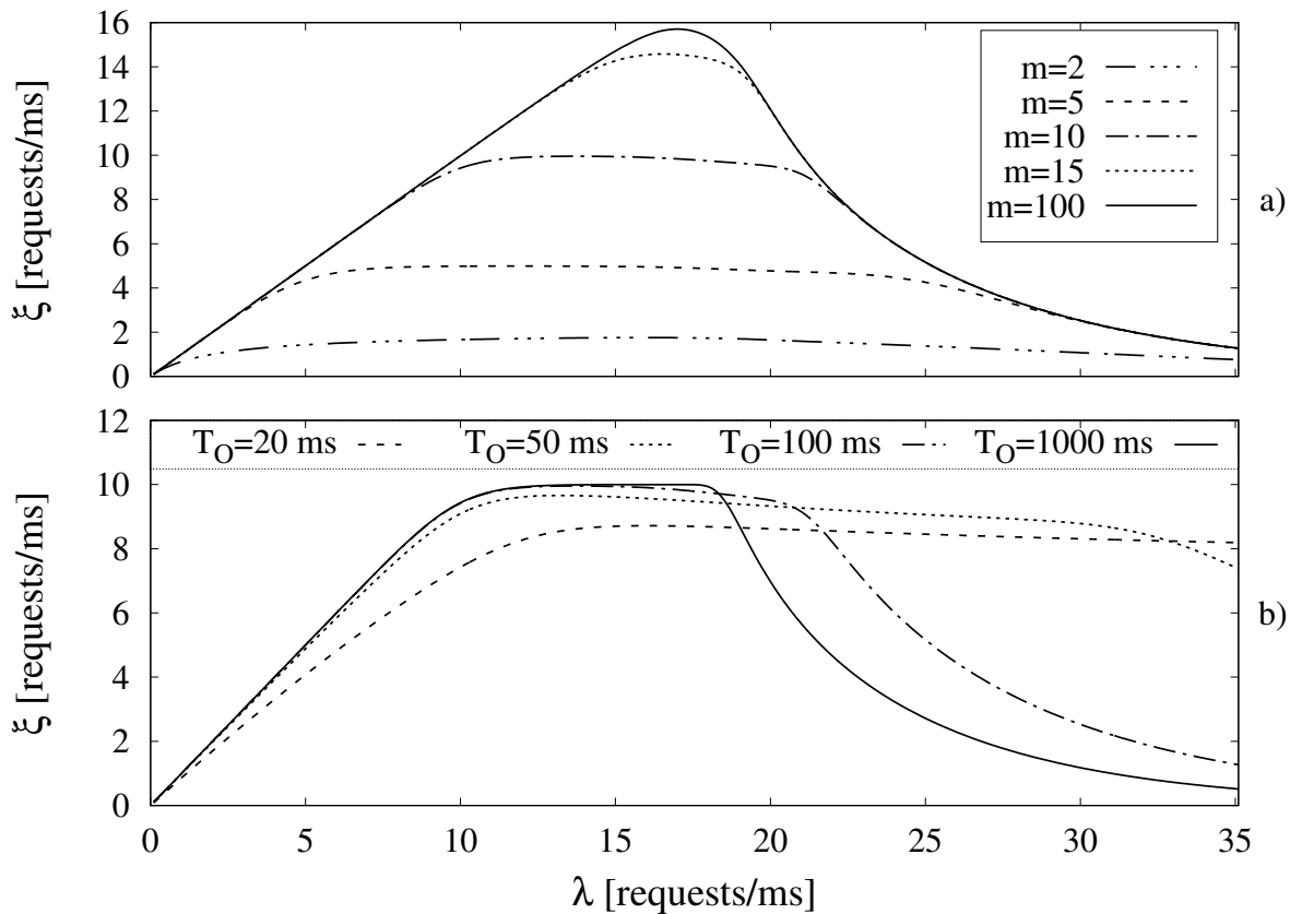
Fig. 7. Effect of varying model parameters on \xi : a) Number of clients served per RAO, m ; b) Timeout
