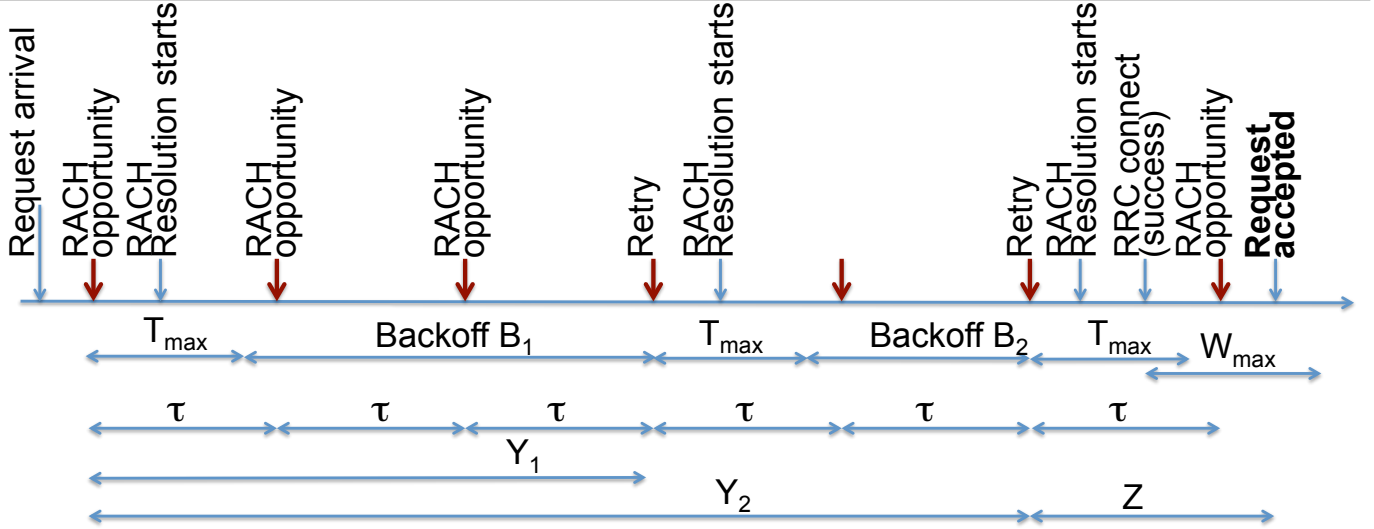
Fig. 1. Timing example for a primary flow request served after 3 attempts.
