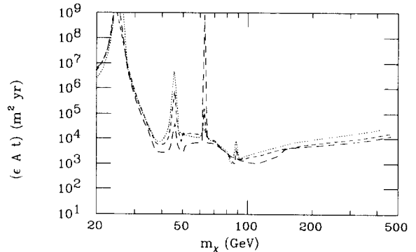
Fig. 14. Effective exposure (\epsilon At) necessary to have a 4\sigma effect with a signal of at least 4 events, as a function of neutralino mass m_\chi . The figure refers to a signal coming from the Sun. The three representative neutralino compositions are P = 0.1 (dotted line), 0.5 (short-dashed line), 0.9 (long-dashed line). The half-aperture of the detector is fixed at 5^\circ from the Sun direction.
