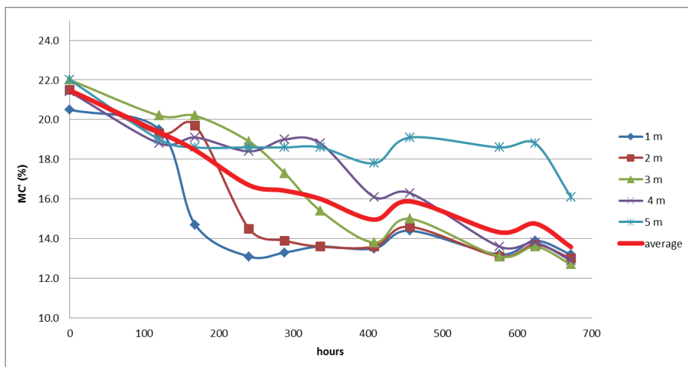
Figure 23 - Trend on MC% evolution inside the bin. 1 m stand for the depth 0-1 m, sampled at 0.5 m, and so on.
