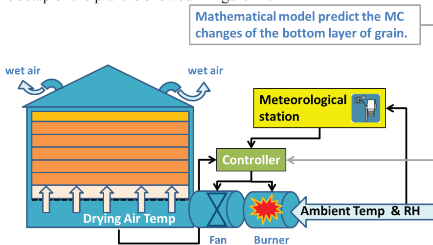
Figure 21- Set up of the low drying temperature plant
