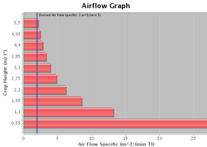
Figure 22- Specific airflow rate calculated for the fan installed at the plant.
