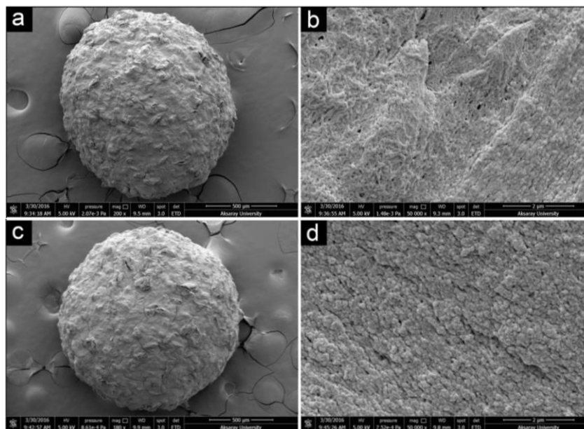
Figure 1. Scanning electron microscope (SEM) images of (a,b) cross linked-chitosan-cellulose composite micro beads; (c,d) green chitosan/cellulose-Pd(II) catalyst. Reprinted from [100]. Copyright (2016), with permission from Elsevier.
