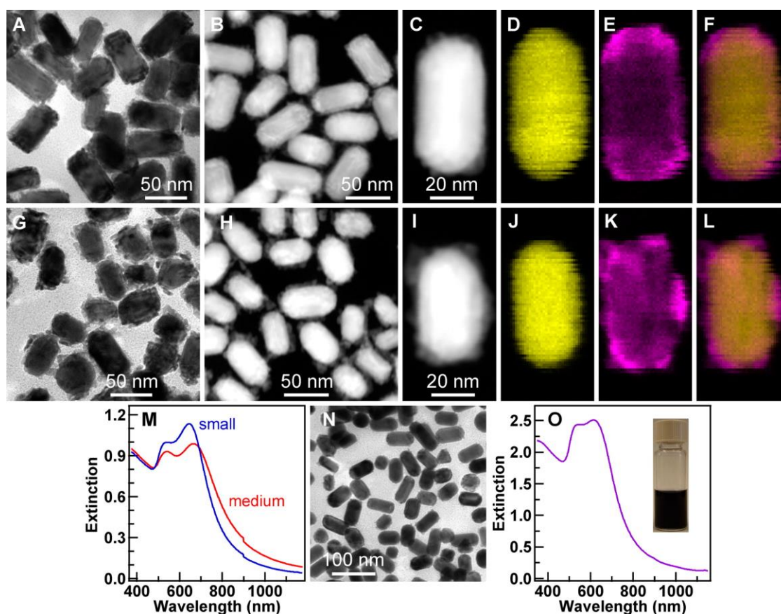
Figure 24. Nanostructures for catalytic reactions under solar radiation. (A–F) Medium Au–Pd nanostructures: (A) TEM image; (B) HAADF-STEM image; (C) HAADF-STEM image of a single nanostructure; (D) elemental map of gold for the nanostructure shown in (C); (E) corresponding elemental map of palladium; (F) merged elemental map; (G–L) Corresponding imaging results for the small Au–Pd nanostructures; (M) Extinction spectra recorded in 0.5 cm cuvettes for the medium and small Au–Pd nanostructure samples; (N) TEM image of the mixture of the medium, small and spherical nanostructure samples; (O) Extinction spectrum of the mixture at 1 cm path length. The inset shows the digital photo of the reaction solution containing the nanostructure mixture in a glass vessel for experiments under solar radiation. Reprinted with permission from [176]. Copyright (2013), with permission from American Chemical Society.
