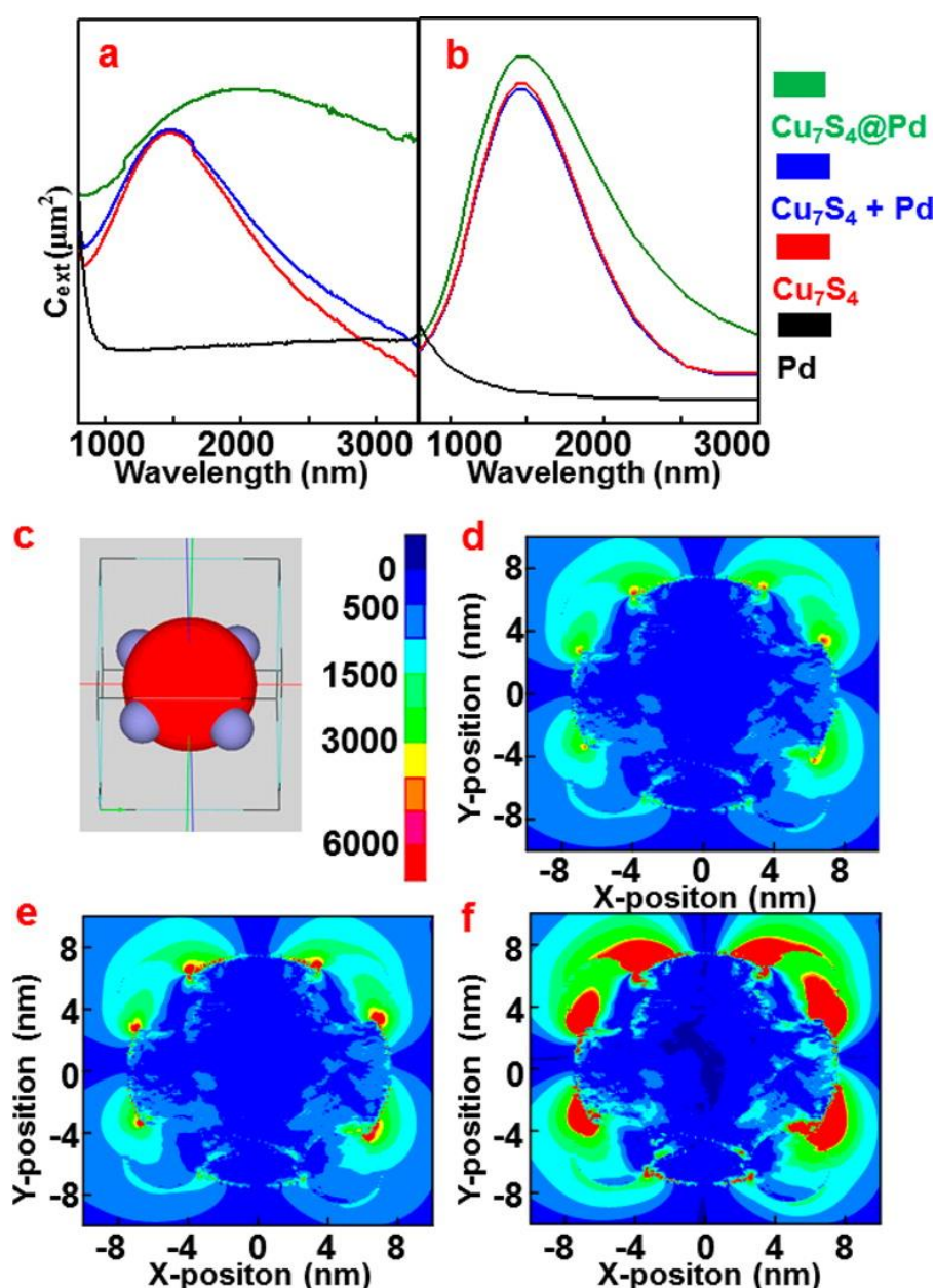
Figure 29. Localized surface plasmon resonance (LSPR) absorption spectra of different nanostructures obtained from experiment (a); and FDTD simulation (b); Green curves: \text{Cu}_7\text{S}_4@\text{Pd} heteronanostructures. Blue curves: physical mixture of \text{Cu}_7\text{S}_4 and Pd nanoparticles. Red curves: \text{Cu}_7\text{S}_4 nanoparticles. Black curves: Pd nanoparticles; (c) FDTD simulation setup for \text{Cu}_7\text{S}_4@\text{Pd} and electrical field intensity scale; (d–f) The 2D contour of the electric field intensities around the \text{Cu}_7\text{S}_4@\text{Pd} heteronanostructures under illumination of 808 nm (d); 980 nm (e); and 1500 nm (f); respectively. Reprinted from [186]. Copyright (2015), with permission from American Chemical Society.
