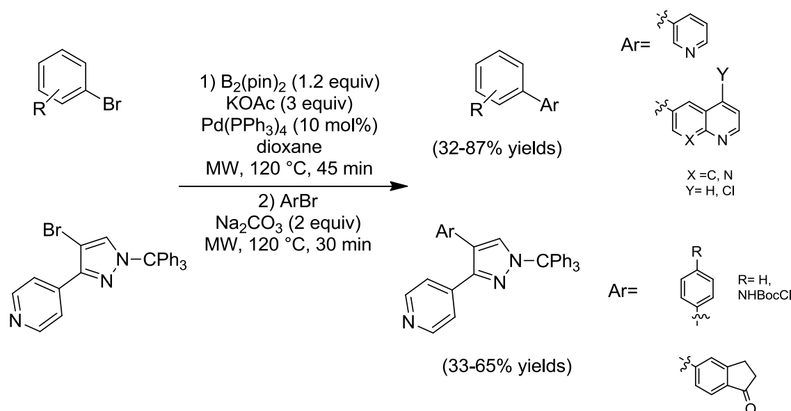
Scheme 28. One-pot borylation/SMC.
