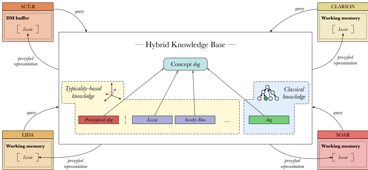
Fig. 3. General overview of the DUAL-PECCS integration within different cognitive architectures.
