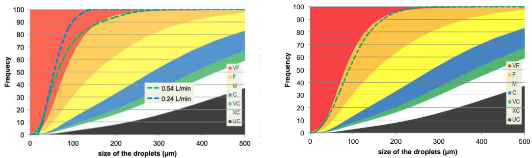
Fig.3.1: Examples of droplets spectra of hot fogger (sx) and knapsack mistblower 1 (dx).
