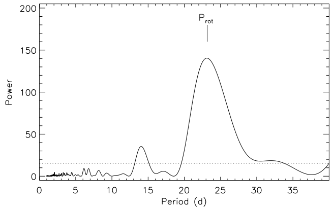
Figure 3. Lomb-Scargle periodogram of the K2 light curve of HD 3167. The horizontal dashed line marks the 0.1% FAP as defined in Scargle (1982).
