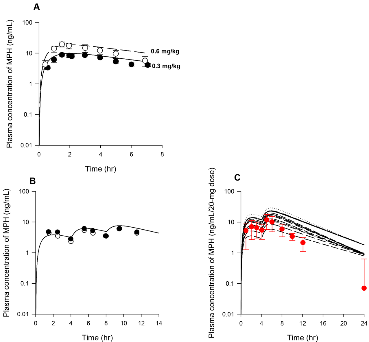
Figure 13. Plasma concentrations obtained after oral dosing of children with MPH. Panel A: Data represent model simulated (dashed line, 0.6 mg/kg; solid line, 0.3 mg/kg) and observed (circles) plasma concentration of MPH after oral dosing with 0.6 mg/kg (○) and 0.3 mg/kg (●) MPH in boys with ADD (n=14) [47]; Panel B: Data represent model simulated (line) and observed plasma concentrations (○, fasting, ●, normal) of MPH normalized to a dose of 5 mg after three repeated oral dosing with 5–15 mg MPH, taken 4 h apart, in children with ADHD (n=14) [48]; Panel C: Data represent model simulated individual (lines) and observed (circles) plasma concentrations of MPH (●) normalized to a dose of 20 mg after two repeated dosing with 10–40 mg MPH, taken 4 h apart, in children with ADHD (n=14) [51]. doi:10.1371/journal.pone.0106101.g013
