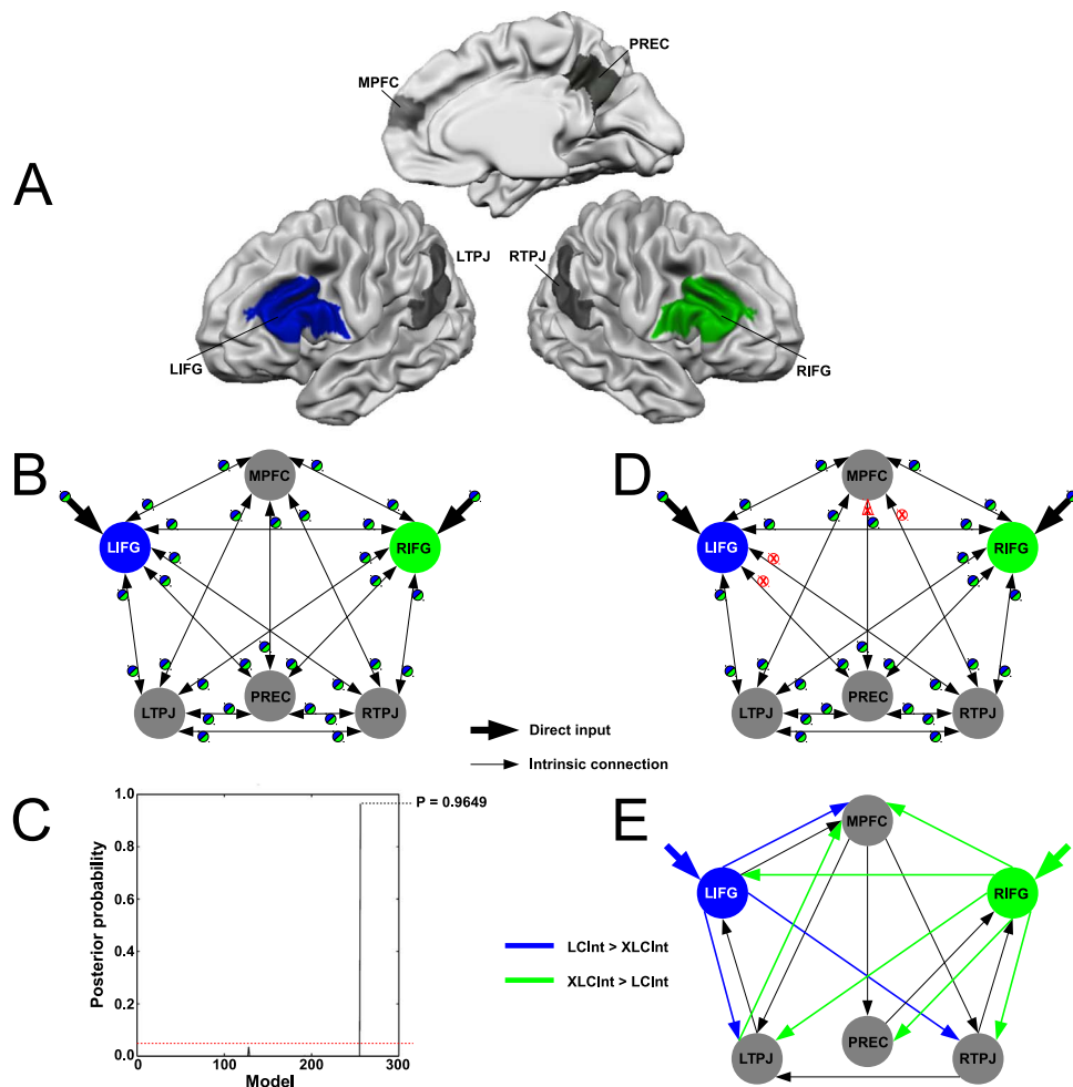
Fig. 1. Dynamic causal model post-hoc optimization. A) Schematic view of the brain regions included in the effective connectivity models, including the four IPN brain regions (MPFC, LTPJ, RTPJ, PREC, all in dark gray), and LIFG (blue) and RIFG (green) as, respectively, the linguistic and extralinguistic input gateways. B) Connectivity architecture of the fully connected model that served as a departure for model optimization. Blue-green circles represent the LCInt versus XLCInt parametric regressor that provided direct psychological input to the model and modulated the inter-regional connections. C) Graph showing the posterior probability of all models generated by the post-hoc optimization. The probability of the optimum model versus the other models. D) Connectivity architecture of the optimum model. The red triangle indicates the only one intrinsic connection pruned by the reduction algorithm, whereas red circles indicate the pruned modulatory connections. E) Schematic connectivity architecture with the significant random-effects parameters of the optimum model. Blue lines indicate stronger direct input (thick arrows) or modulatory (thin arrows) effects induced by LCInt versus XLCInt. Green lines indicate stronger effects induced by XLCInt versus LCInt. Please note that inhibitory self-connections are nowhere represented in this figure. (For interpretation of the references to color in this figure legend, the reader is referred to the web version of this article.)
