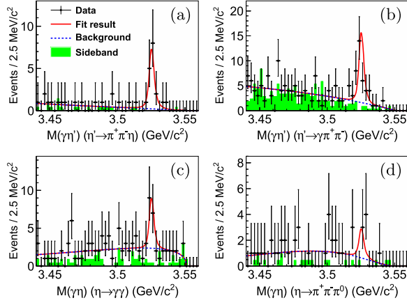
FIG. 2. Results of the simultaneous fits to the two invariant mass distributions of (top) M(\gamma\eta') and (below) M(\gamma\eta) for data. (a) M(\gamma\eta') distribution for h_c \rightarrow \gamma\eta' ( \eta' \rightarrow \pi^+\pi^-\eta ). (b) M(\gamma\eta') distribution for h_c \rightarrow \gamma\eta' ( \eta' \rightarrow \gamma\pi^+\pi^- ). (c) M(\gamma\eta) distribution for h_c \rightarrow \gamma\eta ( \eta \rightarrow \gamma\gamma ). (d) M(\gamma\eta) distribution for h_c \rightarrow \gamma\eta ( \eta \rightarrow \pi^+\pi^-\pi^0 ). The red solid curves are the fit results, the blue dashed curves are the background distributions, and the green hatched histograms are events from the \eta'(\eta) sidebands.
