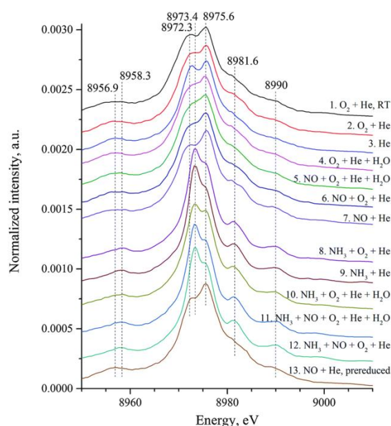
Figure 7. Cu valence-to-core ( K\beta_{2,5} and K\beta'' ) XES spectra of Cu-SSZ-13 catalyst in the course of the NH 3 -SCR reaction and under exposure to the related model gas mixtures at 200 °C. Reproduced with permission from Günter et al. [42]. Copyright (2015) The Royal Society of Chemistry.
