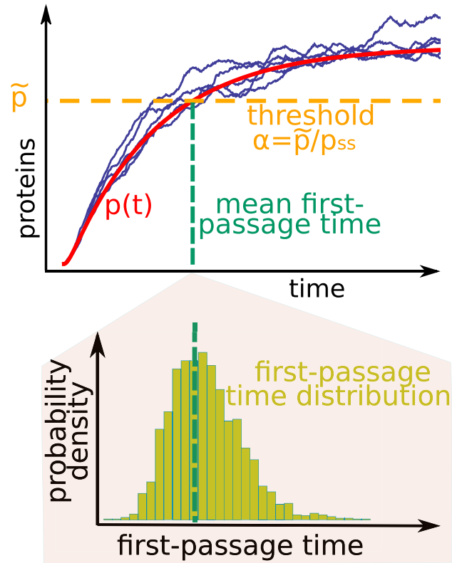
Figure 2. Definition of the threshold-crossing problem. When a gene is switched on at time t = 0 the average protein level (red continuous line) approaches the steady state with the dynamics described by Equation (2). Since gene expression is a stochastic process, individual trajectories fluctuate around the mean behavior, as illustrated by stochastic simulations (blue lines). The distribution of times of crossing a fixed protein level \tilde{p} (orange horizontal dashed line) is the first-passage time distribution (histogram) representing the variability in reaching a certain level of expression. The average first-passage time can be directly deduced from the deterministic mean dynamics (green vertical dashed line).
