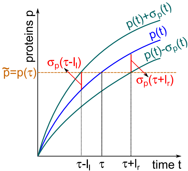
Figure 3. Scheme of the geometric relations at the basis of the analytical estimate of timing fluctuations. The average protein level p(t) rises after induction at time t = 0 . The dynamics depends on the specific regulations acting on the gene. The time evolution of protein fluctuations is captured by the dynamics of the region at one standard deviation from the mean, defined by the curves p(t) \pm \sigma_p(t) . The time necessary to these curves to cross a fixed threshold \tilde{p} gives an estimate of the variability in the first-passage time (FPT).
