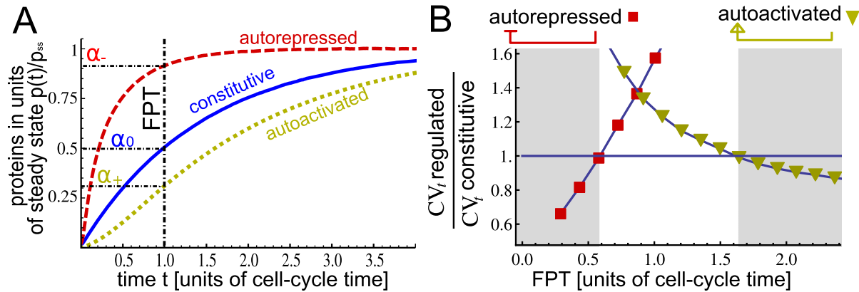
Figure 5. Timing noise can be reduced by different regulatory strategies in different time regimes. (A) Setting of the comparison between regulatory strategies: we imposed the same steady state of expression for the three different circuits. A common average FPT (vertical line) is achieved by placing the target protein level \alpha at a position that depends on the circuit type, corresponding to \alpha_{0,+,-} in this example. Protein and mRNA lifetimes are defined as 5 min and 8 h, while the steady-state number of proteins is ab = 2000 as in Figure 4. The average burst size has a value of b = 5 . The strengths of regulation are defined by the dissociation constants K = 1000 and K = 90 (proteins) for negative and positive autoregulation, respectively. The Hill exponent n = 2 was used for regulations. (B) With the constraints shown in A, the timing noise for autorepression (squares) and autoactivation (triangles) are compared to the timing noise of a constitutive gene as a function of the average FPT value. Given the common final steady-state level of expression, each average FPT (x-axis) corresponds to a different threshold level for the three circuits (as illustrated in panel A) and to a different noise level. When the mean FPT is close to the protein half-life (or to the doubling time for stable proteins) both transcriptional autoregulations increase the timing noise (central region). The two shaded regions show the FPTs for which self-regulation works as a timing noise filter. In particular, autorepression reduces timing noise for time scales shorter than about 0.5 doubling times, while autoactivation is efficient in timing noise reduction on time scales longer than about 1.5 doubling times.
