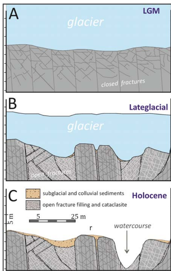
Fig. 12 - Typical morphology of the Plan di Modzjon with rocky rounded ridges (r) and associated wide depressions, which were connected to the progressive evolution of fractures, trenches, minor scarps and counterscarps during glacial erosion. Steps A and B refer to different glacier thicknesses; step C refers to the development of a watercourse in a fracture after glacier retreat.
