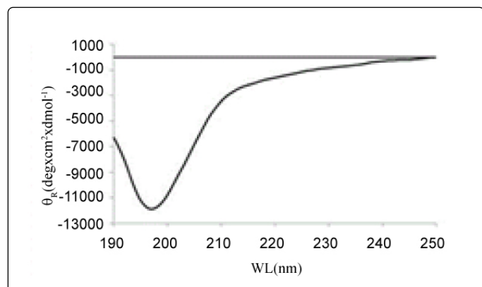
Figure 2: CD spectra of the 75-99 URG7 peptide. A peptide solution 50 μM in 10 mM phosphate buffer pH 6 was analyzed. Data were expressed in terms of [\theta]_R , the molar ellipticity per residue.
