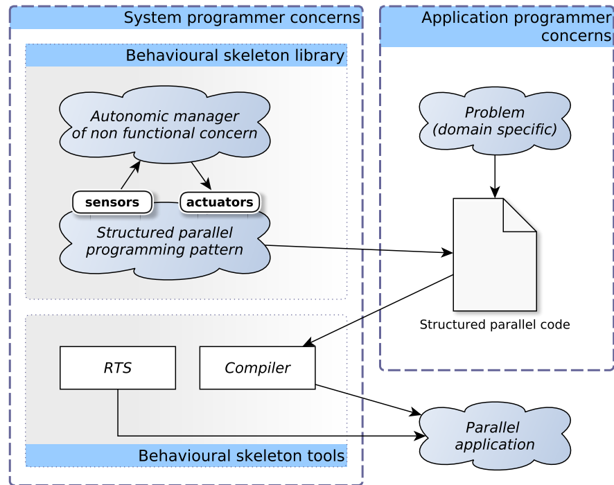
Fig. 3. Behavioural skeletons
