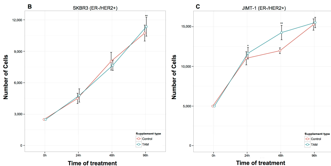
Figure 2. Effects of 1 \mu\text{M} TAM treatment for 24, 48, and 96 h on the proliferation of ER+/HER2+ (A) and ER-/HER2+ (B,C) breast cancer cells. (A) BT474; (B) SKBR3 and (C) JIMT-1. Error bars represent mean standard deviation of 16 separate experiments. Significant differences in treated versus untreated samples are indicated by the p values, * p < 0.05 , ** p < 0.01 .
