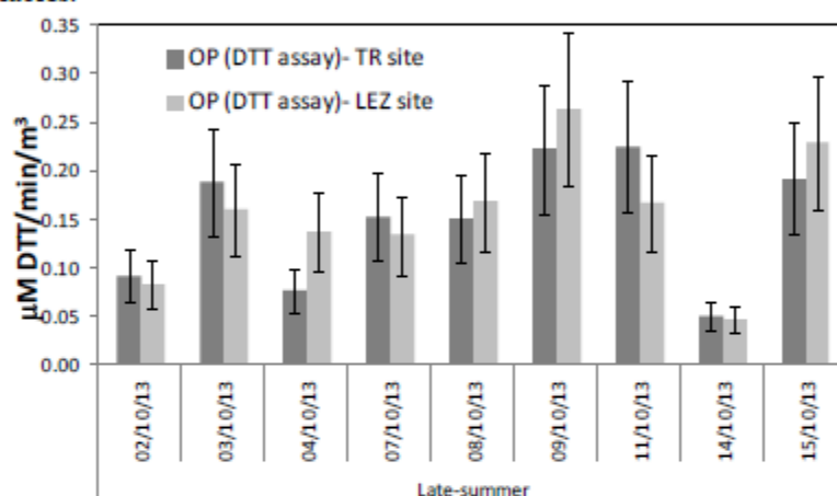
Fig. 2 Daily OP values (OP-DTT) of PM sampled at the TR site and the LEZ site in Milan (1-15 Oct 2013).
