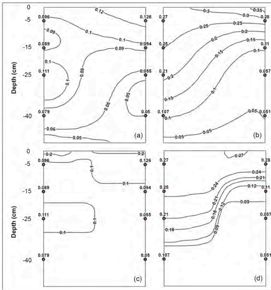
Figure 1. Vertical 2D distribution of soil water content during the center pivot irrigation event before the irrigation ( t_0 ) and at the end of the simulation ( t_1 ). Figures 8a and represent the soil water content interpolated by using thin spline method. Figures (8c and 8d) represent the soil water content distribution simulated by using the ADHYDRA code.
