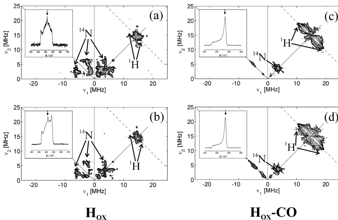
Figure 4. Experimental X-band HSCORE spectra of the H_{ox} (left) and H_{ox-CO} (right) states of the thionine oxidized CaHydA. Spectra (a), (c) refer to the WT protein and (b), (d) to the C298D mutant. The spectra were recorded at field positions corresponding to (a) 341.6 mT, (b) 346.8 mT, (c) 342.2 mT and (d) 347.1 mT, as indicated by the arrow in the echo detected spectra in the insets. The \tau values adopted for the experiments are: (a), (b) \tau = 112 ns; for spectra (c), (d) two spectra recorded at \tau = 136 and \tau = 160 ns were summed together after Fourier transformation. All spectra were recorded at T = 15 K. The simulation analysis of the spectra is reported in the Supplementary Material (Fig. S3 and S4) and the corresponding spin Hamiltonian parameters are listed in Table 2. (2 columns fitting image).
