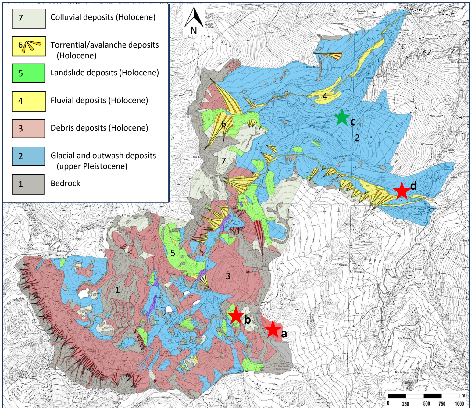
Simplified geological map of the Quaternary succession of the Bulè and Alpetto valleys. The location of the collected jadeitite (sites a, b, d) and eclogite finds (site c) are indicated. Click here to download Figure: Fig. 6.pptx
