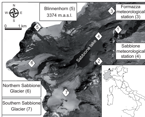
Fig. 1. Digital orthoimage of the study area: 1 and 2, rock glaciers; 3, Formazza meteorological station; 4, Sabbione meteorological station, 5, Blinnehorn peak; 6, Northern Sabbione Glacier; 7, Southern Sabbione Glacier (details in the text). Source: Ministero dell'Ambiente e della Tutela del Territorio e del Mare - Geoportale nazionale, 2006 (wms service available at: http://wms.pcn.minambiente.it/ogc?map=/ms_ogc/WMS_v1.3/raster/ortofoto_colore_06.map ).
