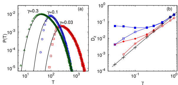
FIG. 12. (Color online) Exit time statistics. (a) Exit time PDF for \Psi = 1.1 , and \Phi = 0.05 at three turbulent intensities \gamma as labeled, compared with the prediction (21) with D_z and V_d obtained as explained in the text. (b) Vertical diffusivity constant D_z estimated from exit time statistics for cells with \Phi = 0.05 (red circles) and \Phi = 0.2 (blue squares) for \Psi = 1.1 (filled symbols) and \Psi = 1.5 (empty symbols). Statistical convergence is poor at large and small \gamma 's for \Phi = 0.05 . The solid black line displays the \gamma^2 behavior of the turbulent diffusivity measured along tracer trajectories (plus symbols).
