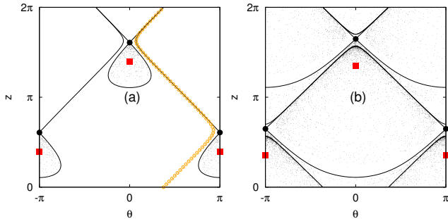
FIG. 2. Cells positions in the laminar 2D Kolmogorov flow at a long time on the (\theta, z) torus for (a) \Psi = 1.06 and (b) \Psi = 1.12 with \Phi = 0.2 , corresponding to Fig. 1b and c, respectively. Black circles (red squares) mark the hyperbolic (elliptic) fixed points (17). Black curves denote the separatrices emerging from the hyperbolic fixed points, which are obtained from the isolines of \mathcal{H} computed at H1 and H2 . At \Psi < \Psi_c (a) small black dots corresponds to trapped orbits and empty circles to the orbit (15) which asymptotically characterized the vertically migrating cells and is very close to the separatrix. For \Psi > \Psi_c (b) all orbits are trapped.
