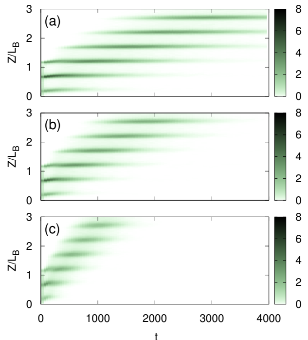
FIG. 5. (color online) Evolution of the vertical number density \rho(Z, t) in the 2D laminar Kolmogorov flow with parameter as in Fig. 1c and the presence of rotational Brownian motion with (a) Pe_r^{-1} = 0.005 , (b) 0.01, and (c) 0.04.
