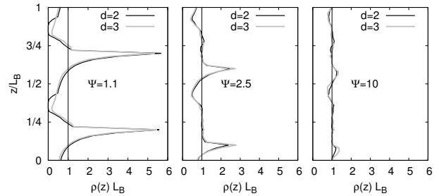
FIG. 4. Number density of algae corresponding to the two layers restricted to the domain z \in [0 : L_B] , for both 2D and 3D for \Phi = 0.05 and three values of \Psi as labeled. Density differs for minor details in the two cases. Notice that layers tend to disappear for large \Psi .
