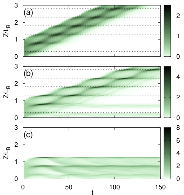
FIG. 1. (color online) Evolution of the vertical density of cells, \rho(Z, t) , in the 2d laminar Kolmogorov flow for \Phi = 0.2 with (a) \Psi = 0.9 < \Psi_c , (b) 1 < \Psi = 1.06 < \Psi_c and \Psi = 1.12 > \Psi_c , where \Psi_c is given by (16). Dotted horizontal lines in (a) and (b) mark vertical velocity minima (see text for a discussion). The density has been obtained coarse-graining the vertical position of N = 10^4 cells initialized uniformly in (\theta, Z) \in [-\pi, \pi] \times [0 : 2\pi] and evolved by integrating Eqs. (12) and (13) with a 4 th -order Runge-Kutta scheme.
