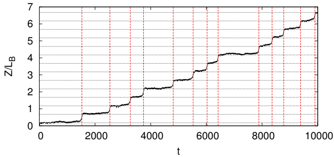
FIG. 6. (Color online) Typical cell trajectory for \Phi = 0.05 , \Psi = 1.12 and Pr_r^{-1} = 0.005 . We can identify two regimes: temporary trapping in a layer (around the horizontal dashed lines demarking the elliptic points) and short jumps between layers. Vertical (red) lines mark the transition between adjacent layers, numerically identified as the times at which the vertical position Z increases of L_B/2 .
