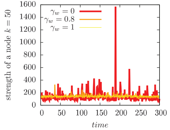
FIG. 6. (Color online) Strength of a randomly chosen node of degree 50 in ( \gamma_k = 0, \gamma_w = \{0, 0.8, 1\} ) networks with \eta = 1 fraction edge weights permuted at each time step.
