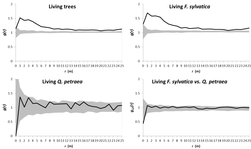
Fig.1. Tree spatial patterns quantified with the pair correlation function g(r) for the overall living tree population and for each species separately. In the lower right graph, bivariate pair-correlation function g_{12}(r) between the two species. Critical bands from the Monte Carlo simulations are shaded ( p < 0.01 ).
