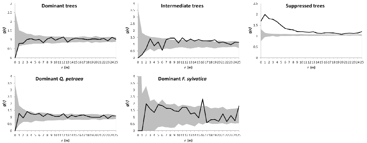
Fig.3. Univariate analyses of the spatial pattern of trees belonging to different layers, considering all the species together and separately, using the pair-correlation function g(r) . Critical bands from the Monte Carlo simulations are shaded ( p < 0.01 ).
