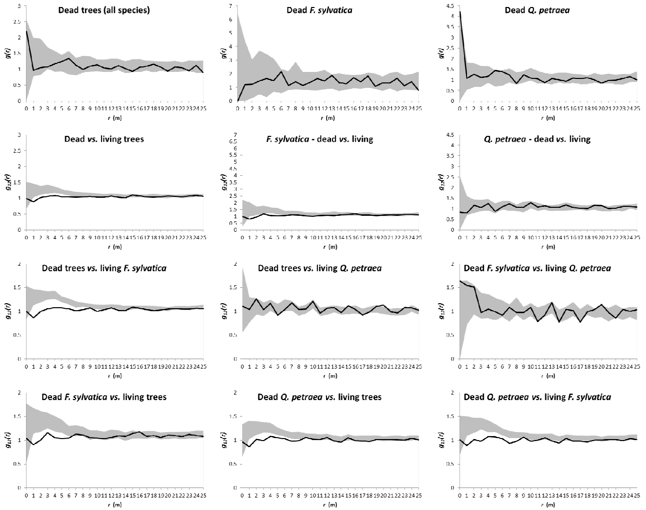
Fig.2. Univariate analyses ( g(r) ) on the spatial patterns of dead trees and bivariate analysis ( g_{12}(r) ) of their spatial interaction with living trees under the random mortality null model. Critical bands from the Monte Carlo simulations are shaded ( p < 0.01 ).
