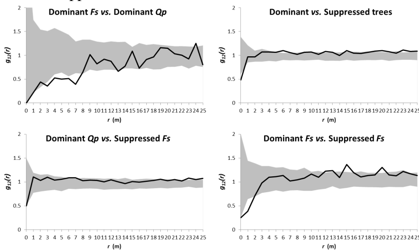
Fig.4. Bivariate analyses of the spatial interaction between trees belonging to different layers, considering all the species together and separately, using the pair-correlation function g_{12}(r) . Critical bands from the Monte Carlo simulations are shaded ( p < 0.01 ).
