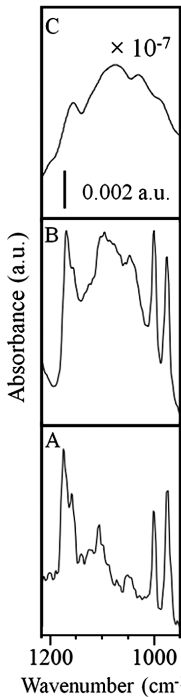
Figure 4. Absorbance FTIR spectra in the range of 1200–950 \text{cm}^{-1} of: (A) pristine PP fiber; (B) PP fiber functionalised with antibiotic chitosan/CFC coating and (C) chitosan reference powder. Spectra A and B were collected in the ATR mode, whereas spectrum C in transmission mode.
