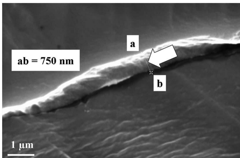
Figure 2. Cross-section of the PP fiber functionalised with chitosan/CFC coating. The arrow indicates the maximum thickness of the coating between the points a and b.
