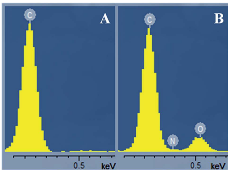
Figure 3. EDS spectra of plasma-activated PP fibers (section A) and chitosan/CFC coated fibers (section B).
