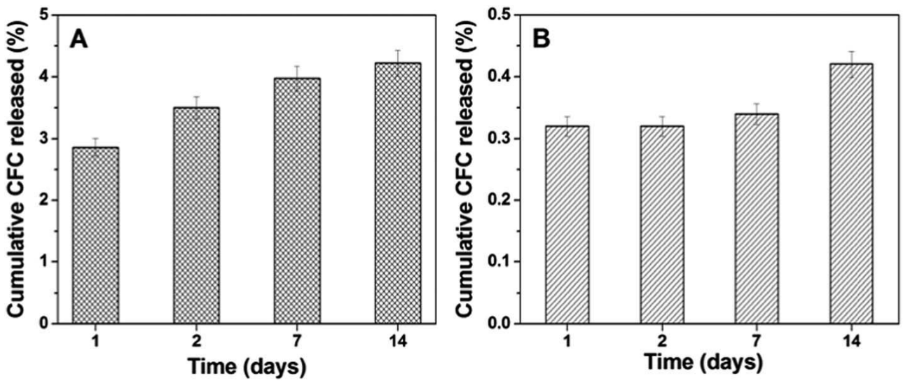
Figure 6. CFC release (%) from MA (section A) and MB (section B) meshes vs. residence time (days) in PHY solution.
