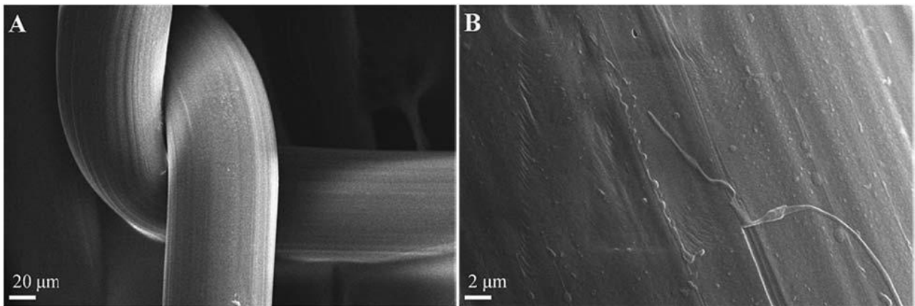
Figure 1. SEM micrographs of the PP fiber functionalised with the chitosan/CFC antibiotic coating at low (A) and high (B) magnifications.
