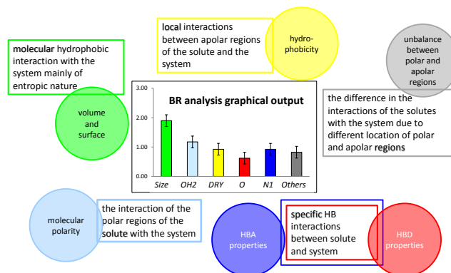
75 Fig. 1. BR analysis: interpretation scheme. A typical graphical output is shown in the center. The solutes' properties described by the blocks are in circular frames. The main interactions in which any block is involved are in rectangular boxes. A color code is always associated to any block (green for Size, cyan for OH2 (Water), yellow for DRY, blue for N1, red for O and grey for Others).
